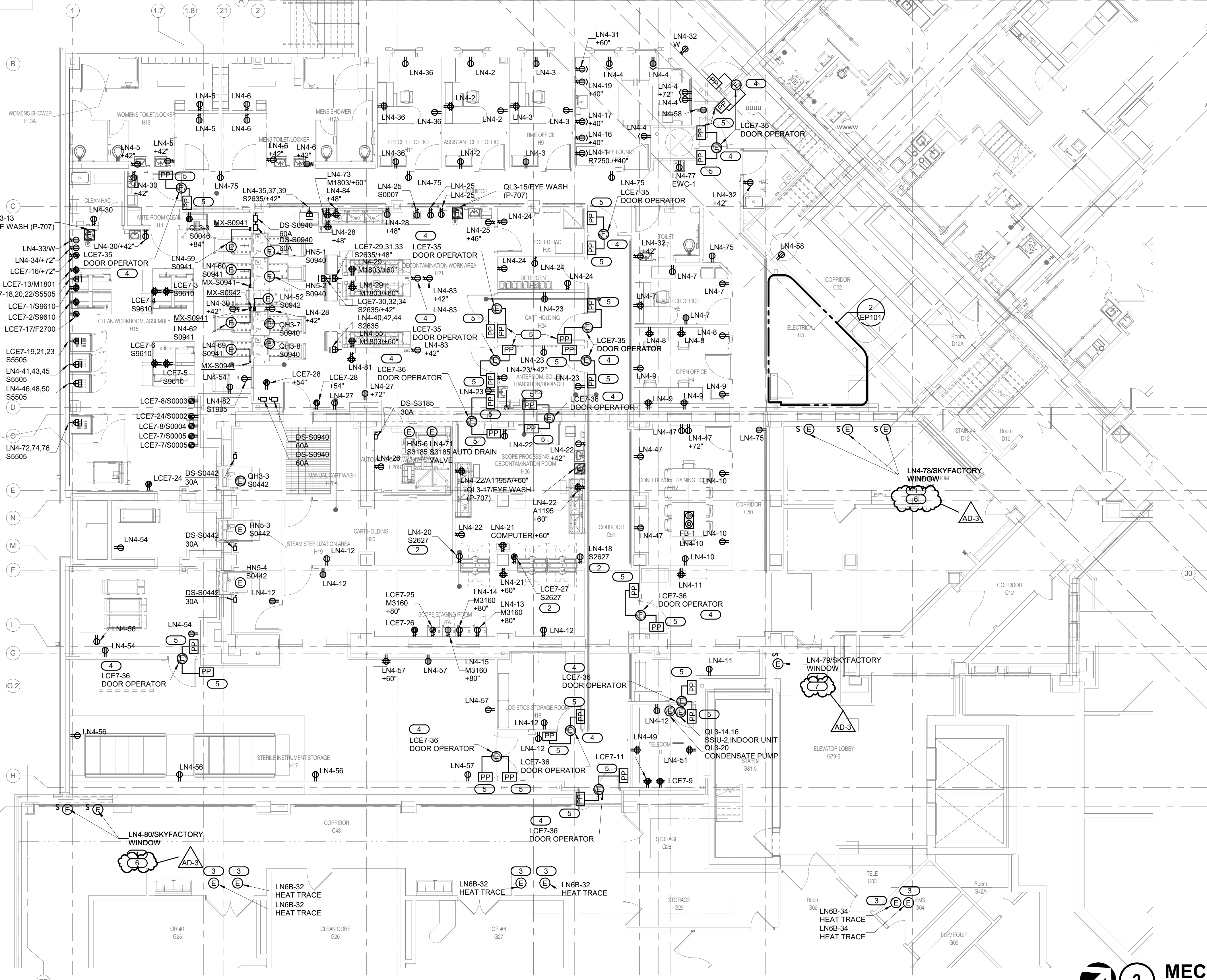
1 GROUND LEVEL FLOOR PLAN - POWER 1/8" = 1'-0"
