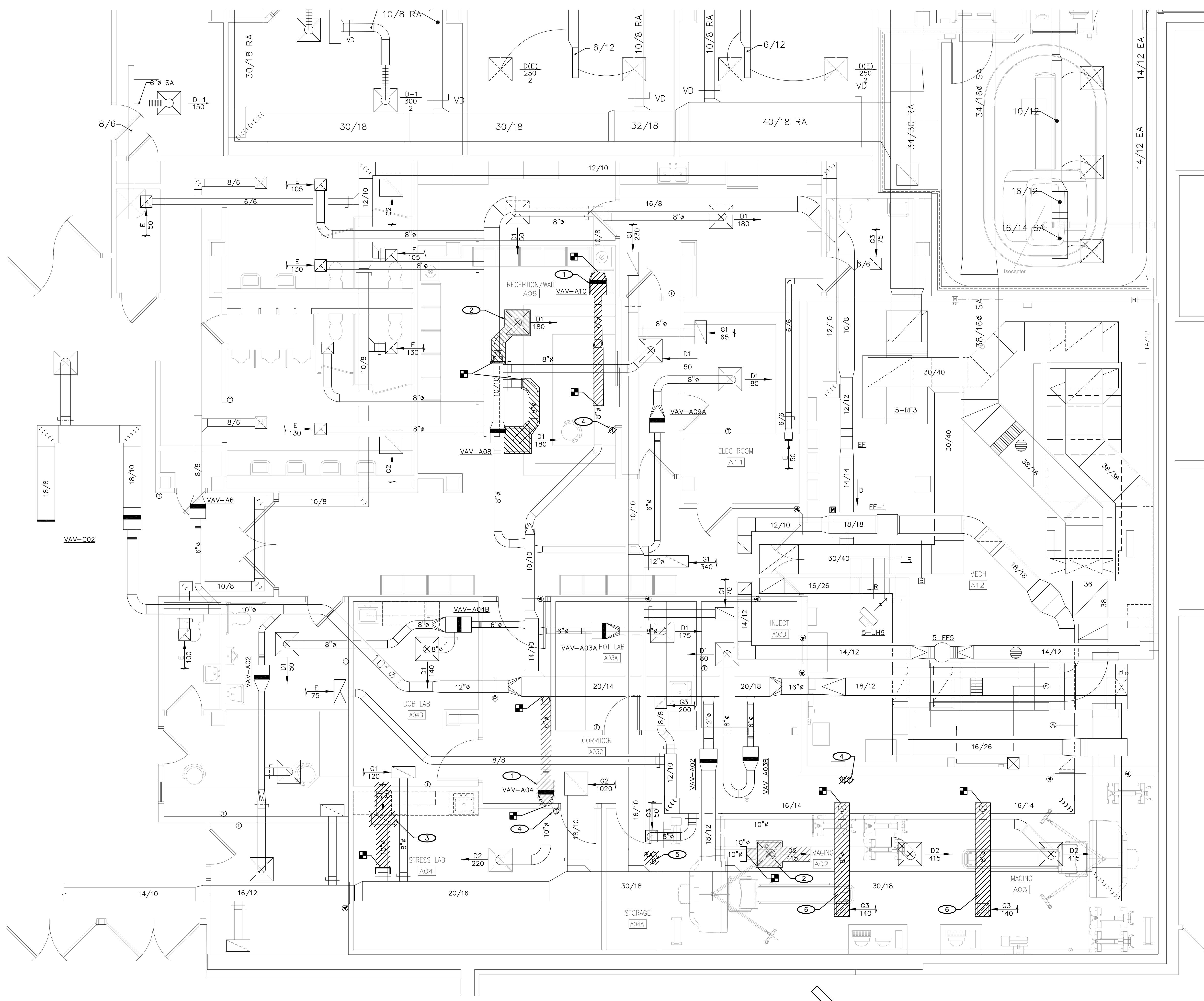
(2F) NUCLEAR MEDICINE AREA MECHANICAL DEMOLITION PLAN SCALE: 1/4" = 1'-0"
