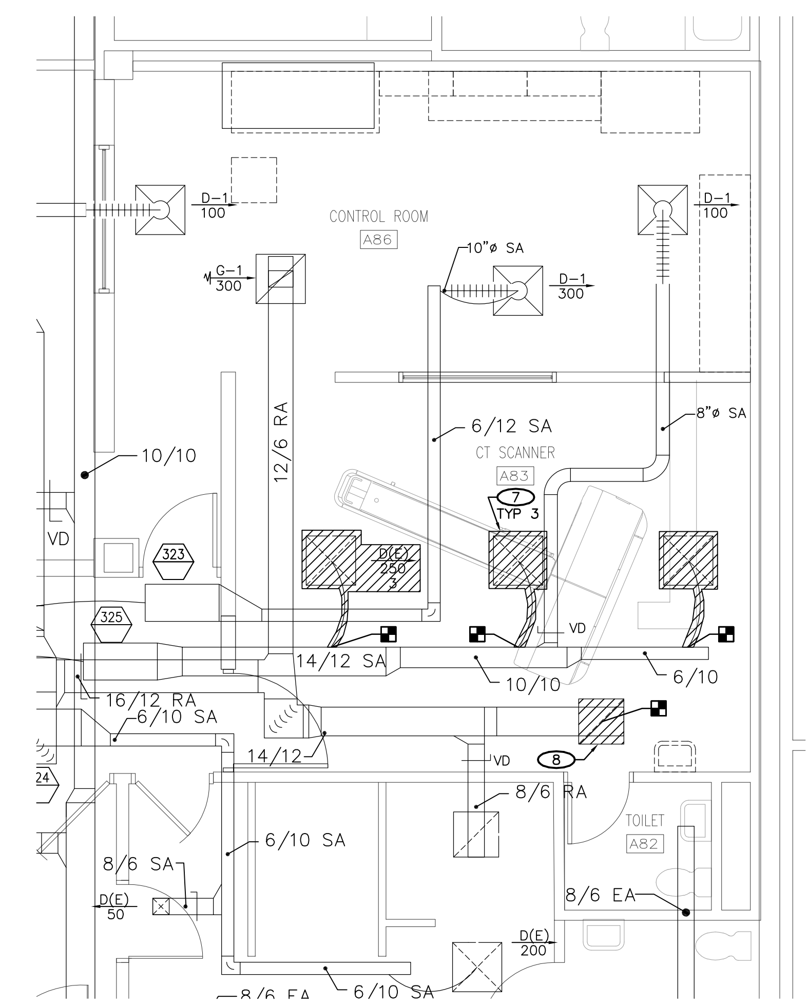
(8C) CT SCANNER AREA MECHANICAL DEMOLITION PLAN SCALE: 1/4" = 1'-0"
