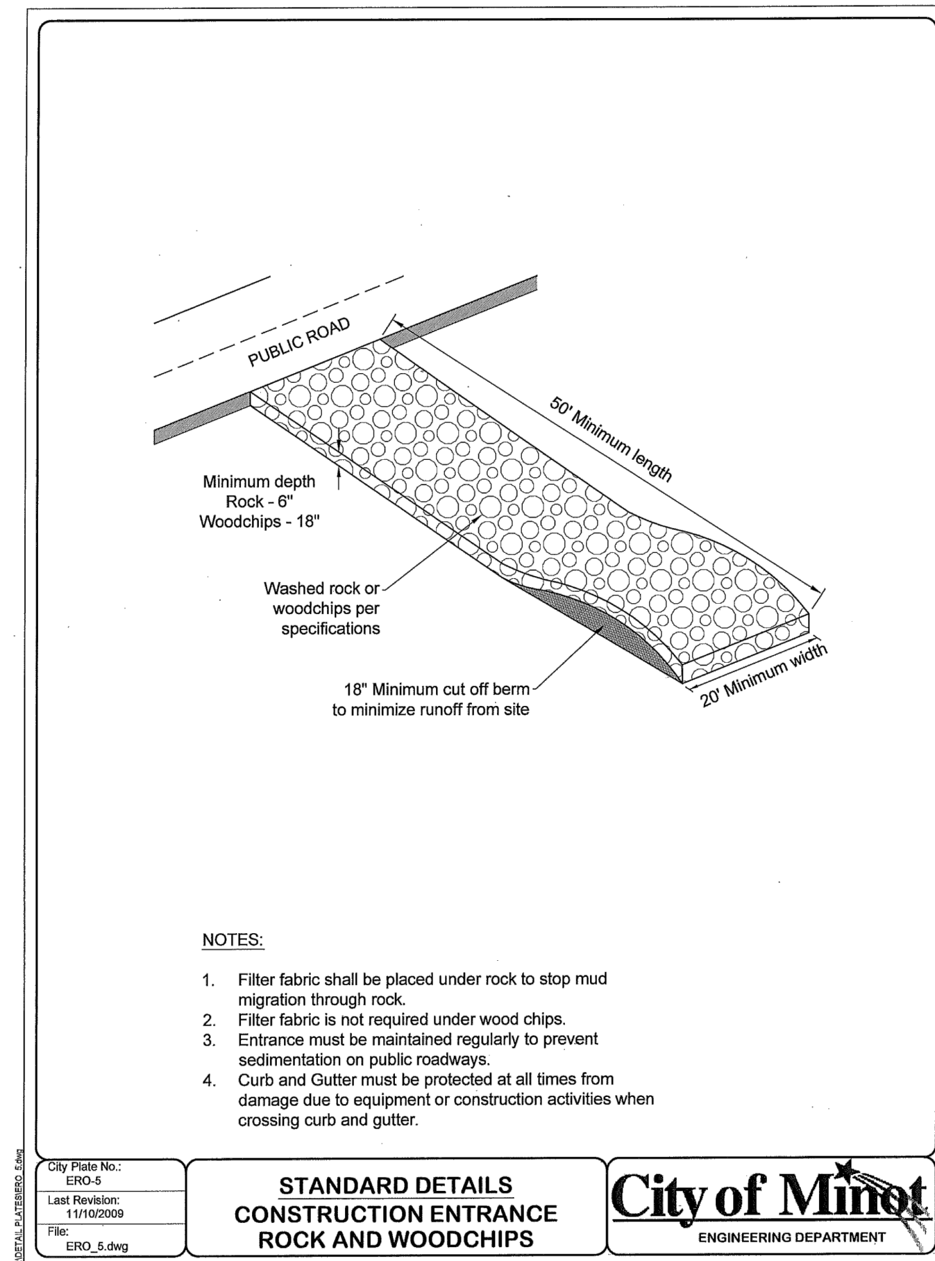
C1 CONSTRUCTION ENTRANCE ROCK AND WOODCHIPS
