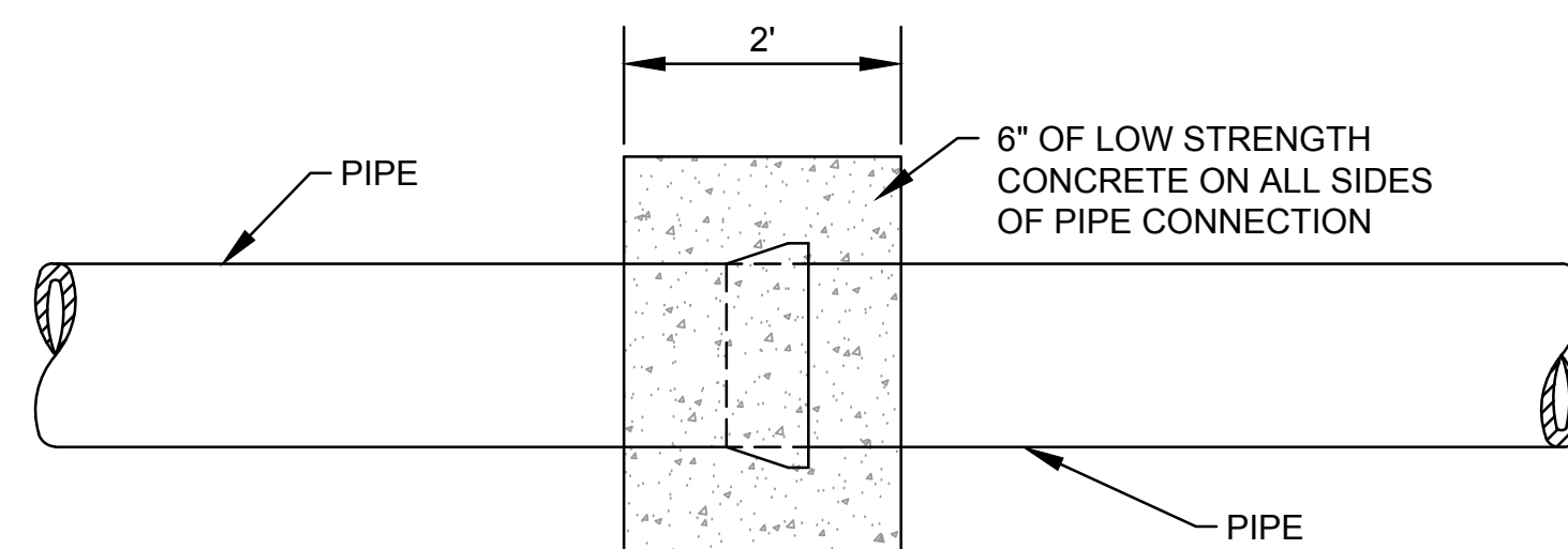
C3 PIPE TO PIPE CONNECTION DETAIL NTS
