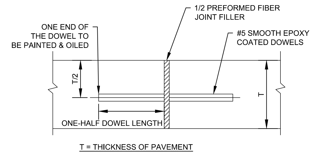
C4 TYPE F - DOWELED CONTRACTION JOINT NTS
