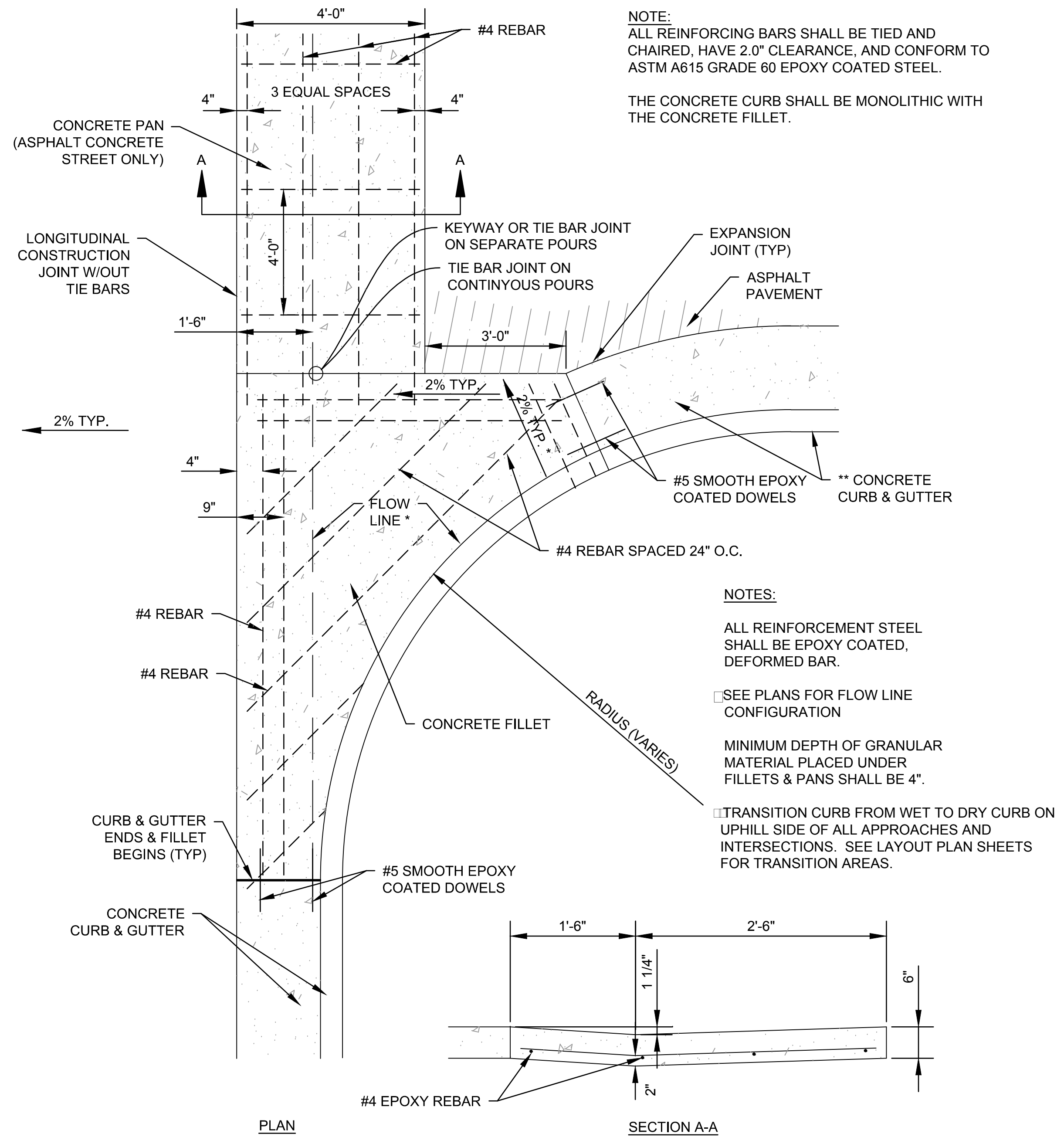
C2 REINFORCED PORTLAND CEMENT CONCRETE FILLET & PAN NTS
