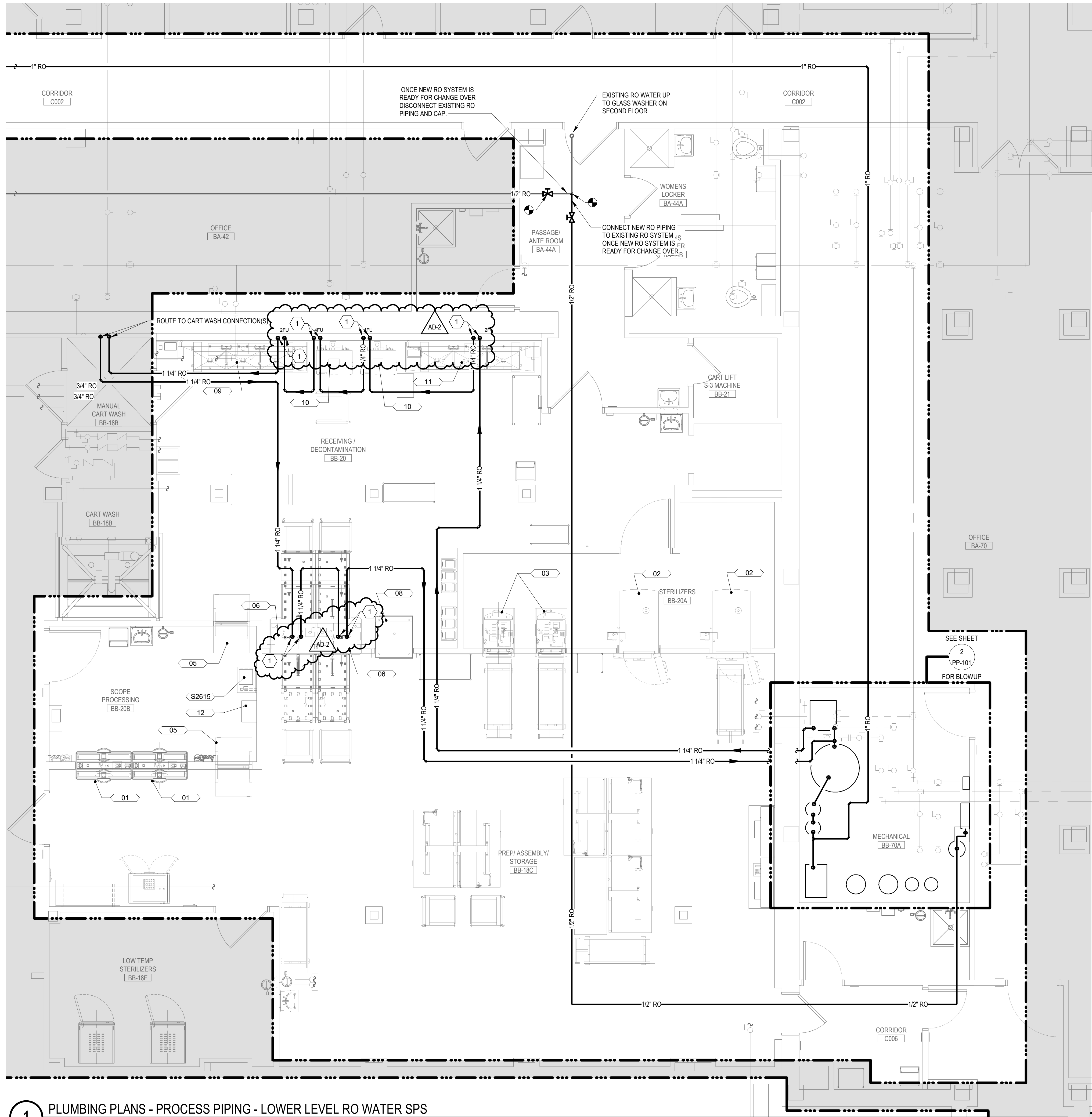
1 PLUMBING PLANS - PROCESS PIPING - LOWER LEVEL RO WATER SPS 1/4" = 1'-0"
