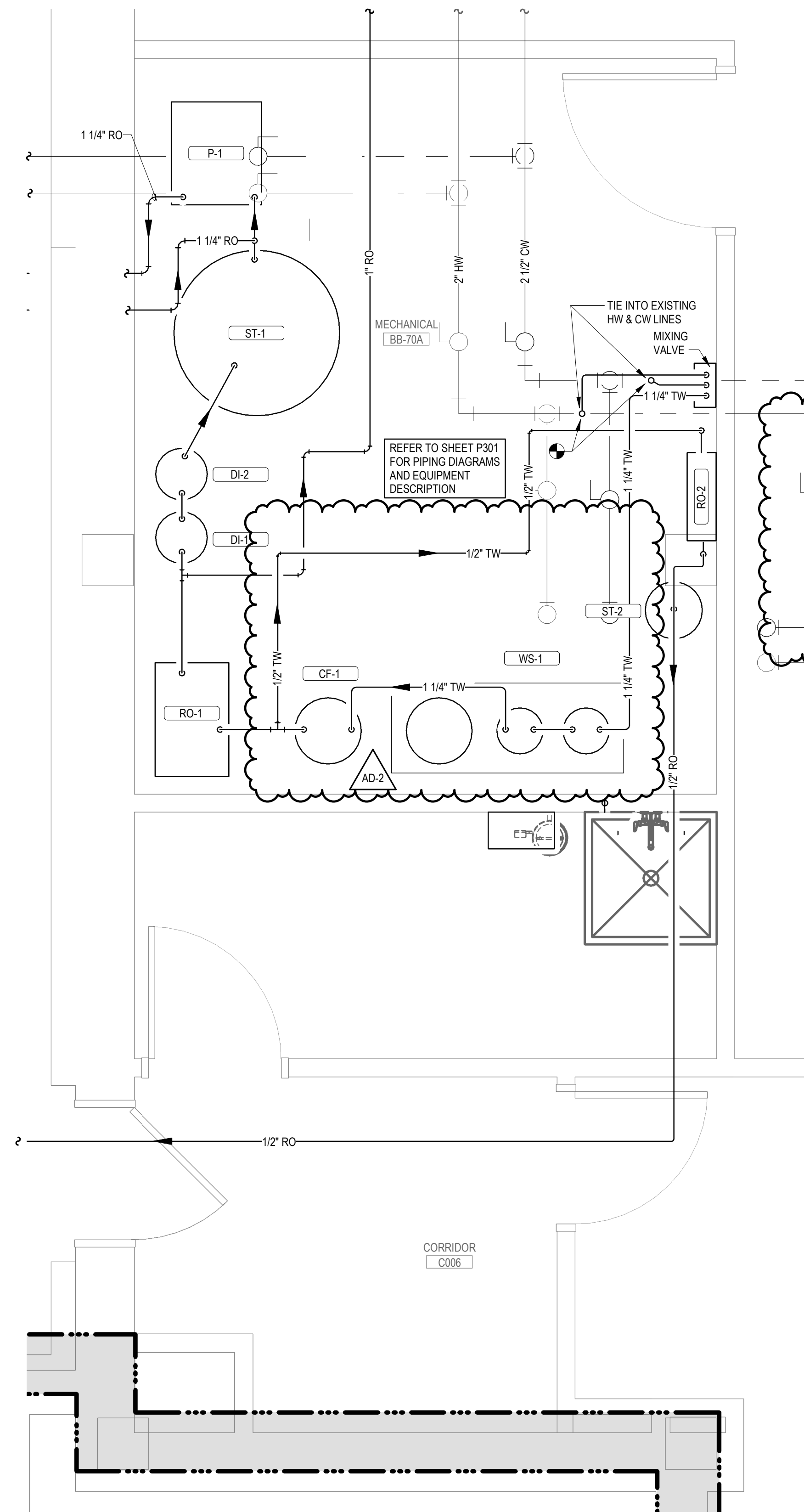
2 LOWER LEVEL - ENLARGED RO MECH ROOM 1/2" = 1'-0"
