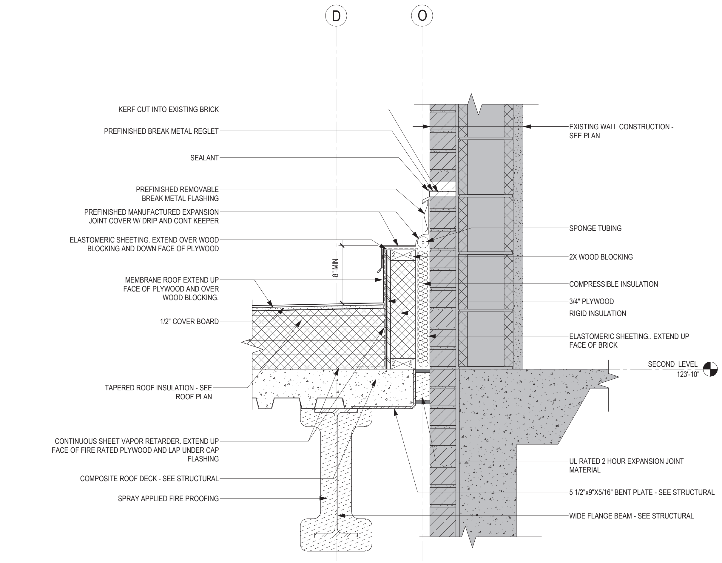
2 ROOF DETAIL - MEMBRANE ROOF @ EXISTING SECOND LEVEL 1 1/2" = 1'-0"
