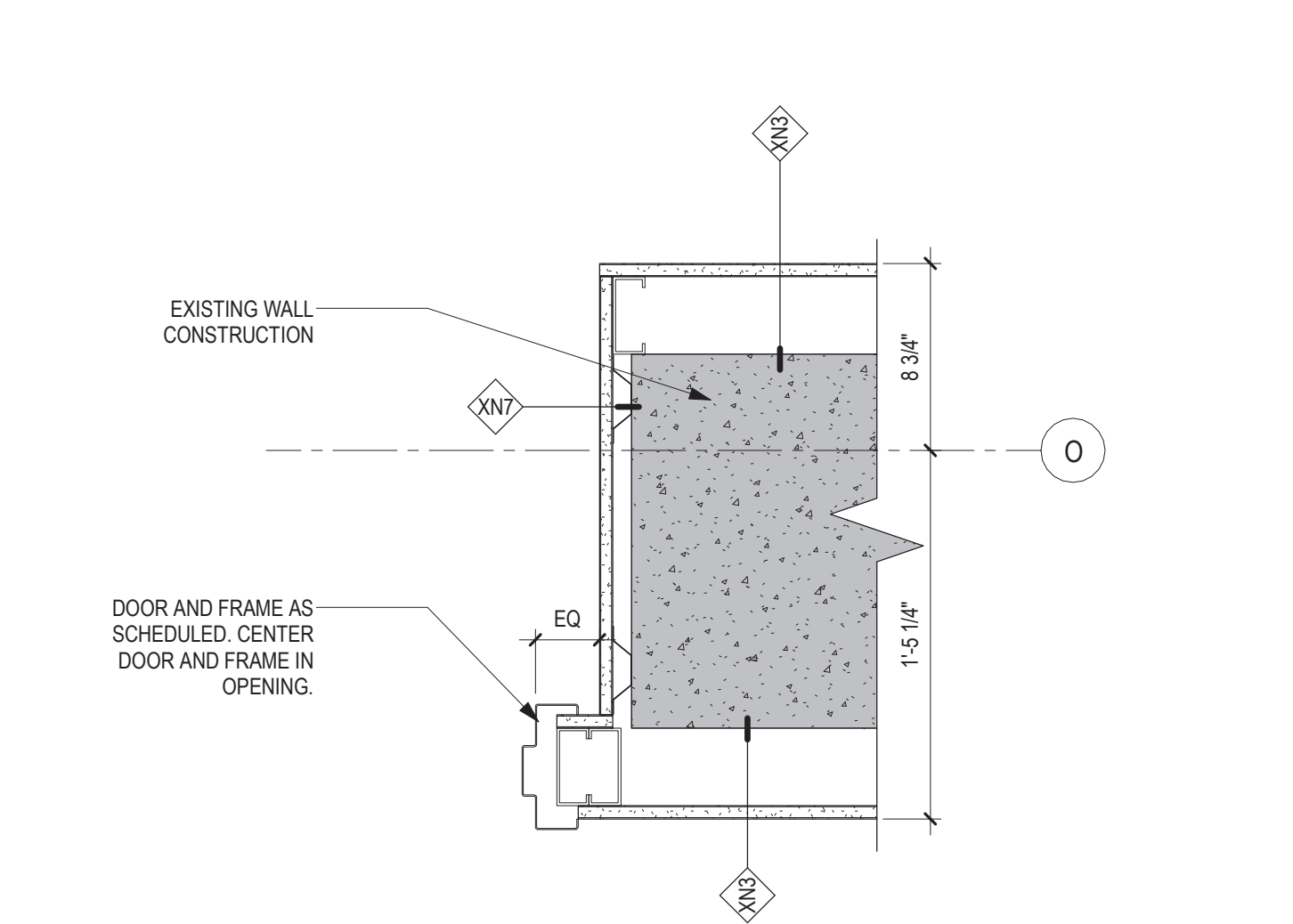
7 PLAN DETAIL - PARTITION AND DOOR JAMB AT DOOR H26B 1 1/2" = 1'-0"
