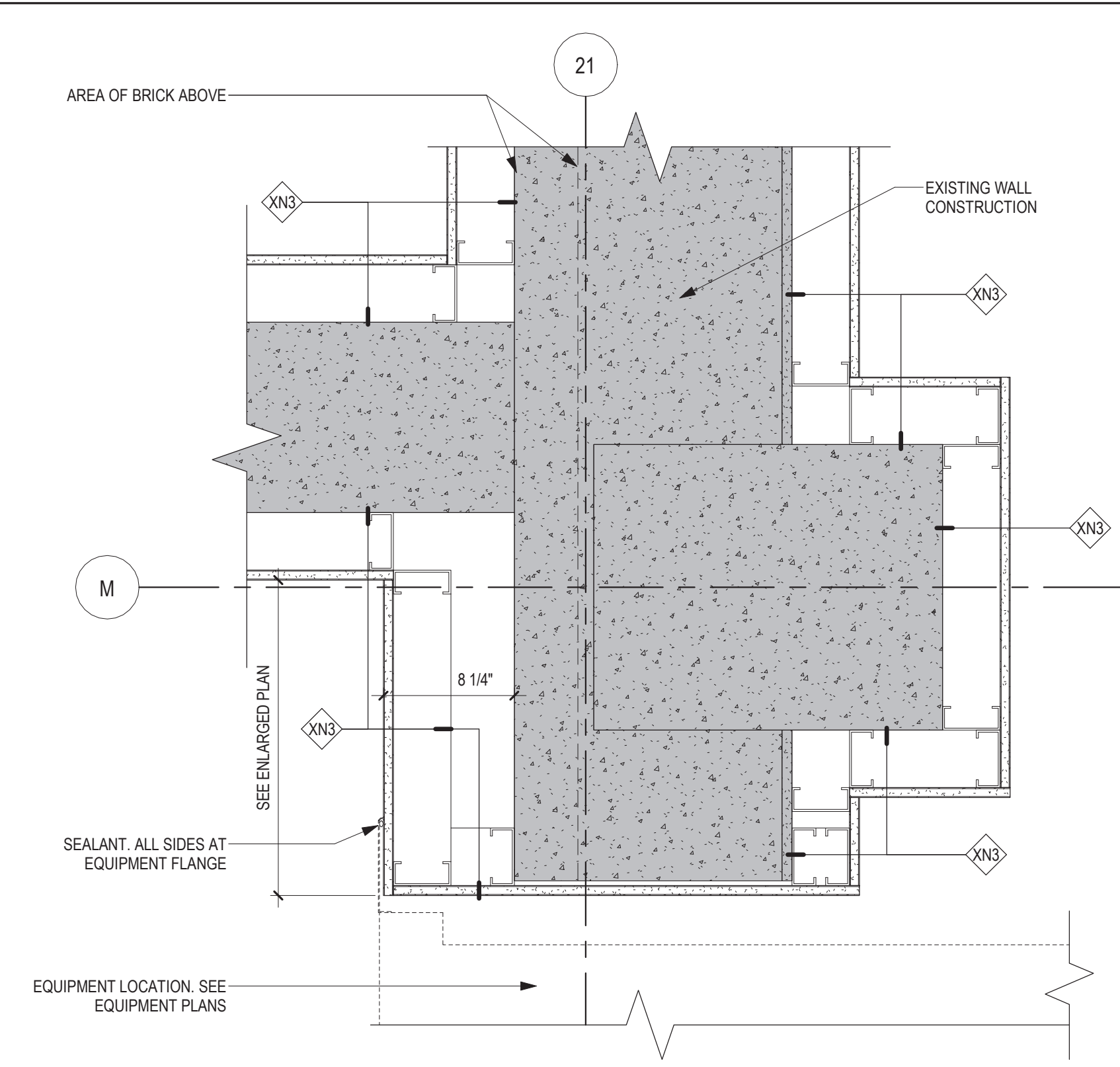
3 PLAN DETAIL - PARTITION OPENING AT STEAM STERILIZER 1 1/2" = 1'-0"
