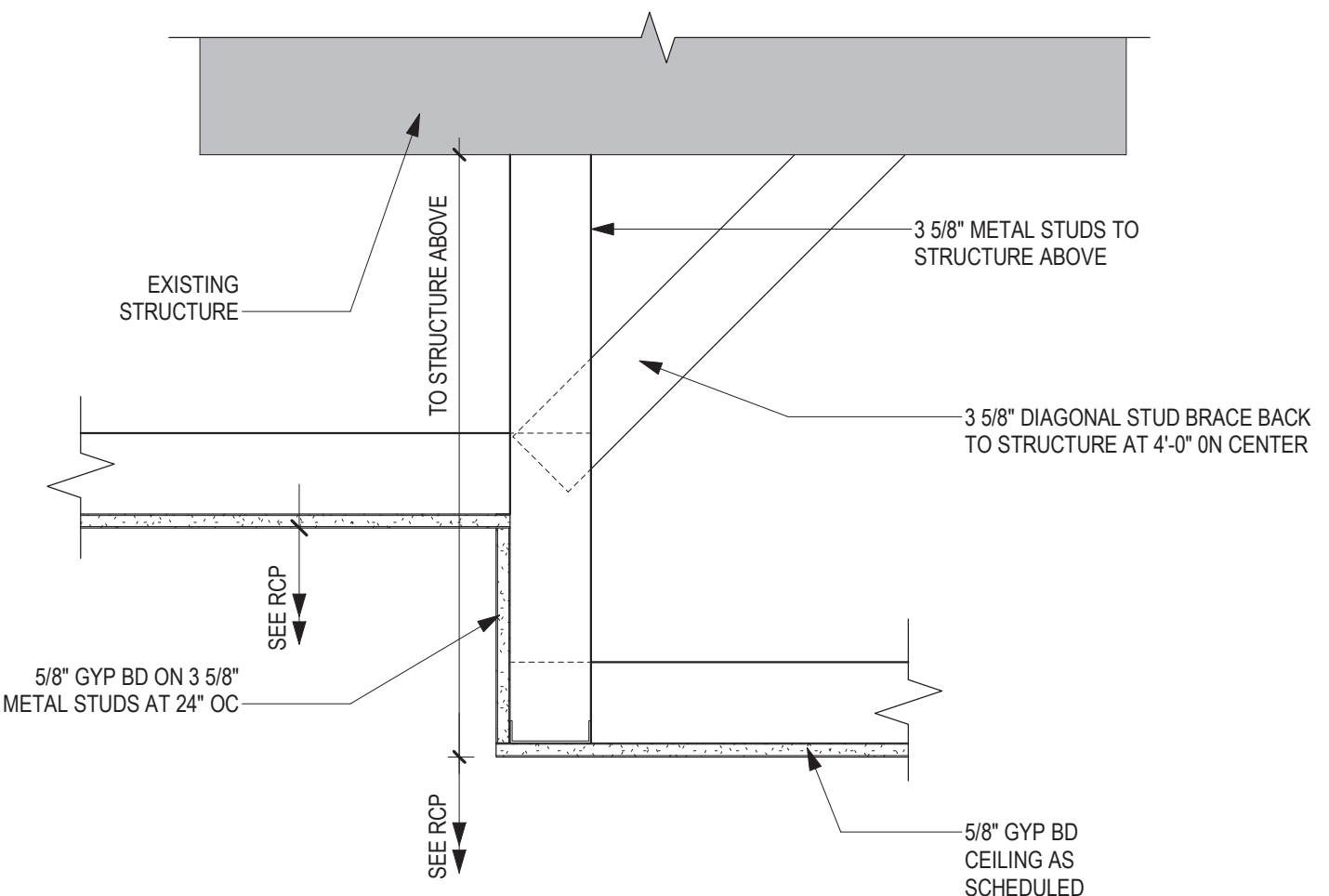
SECTION DETAIL - GYP BD CEILING TO GYP BD CEILING 1 1/2" = 1'-0"
