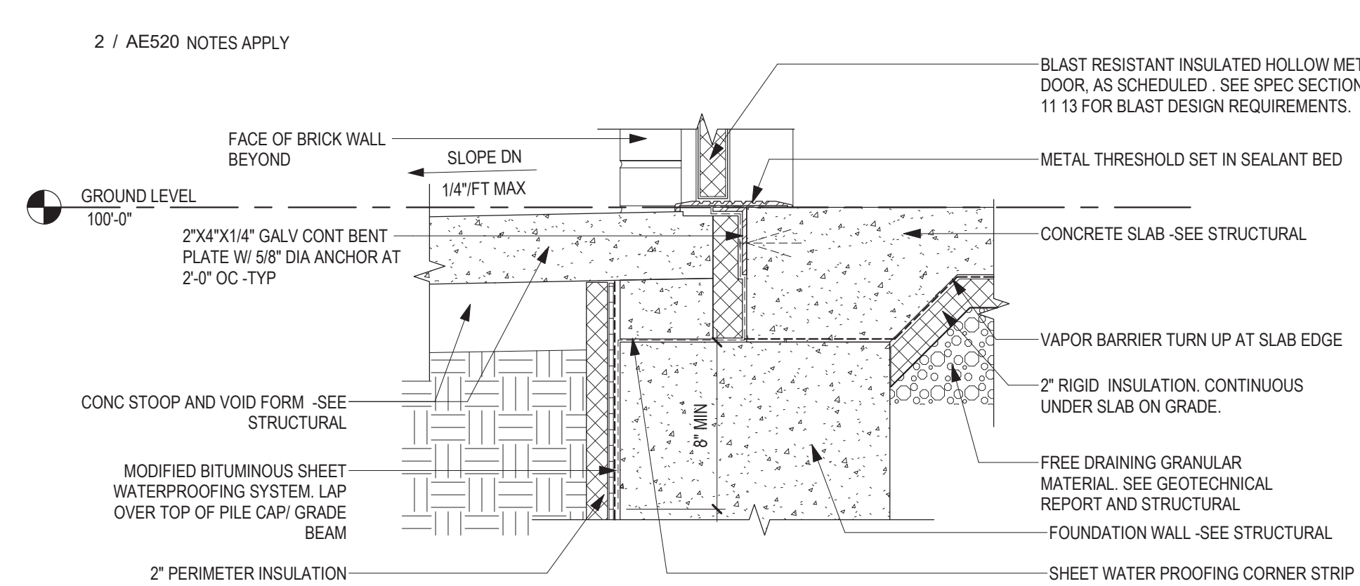
6 SECTION DETAIL EXTERIOR - DOOR SILL 1 1/2" = 1'-0"
