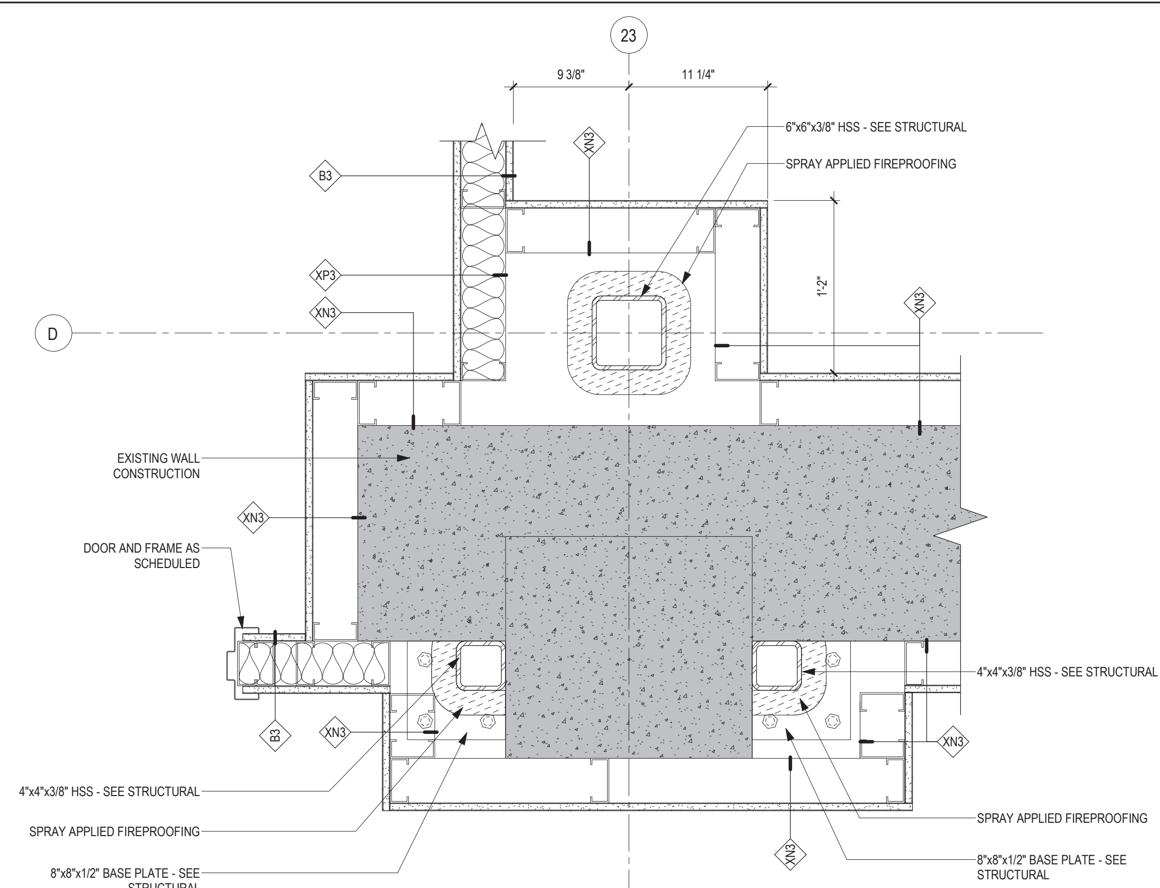
4 PLAN DETAIL - PARTITION @ COLUMN D-23 1 1/2" = 1'-0"
