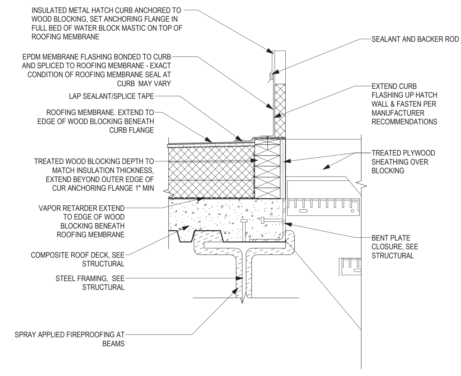
2 ROOF DETAIL - ROOF HATCH CURB 1 1/2" = 1'-0"
