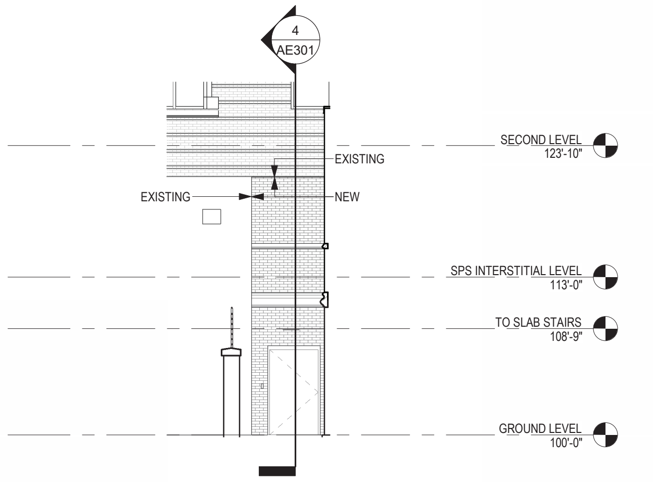
3 PARTIAL EXTERIOR ELEVATION - WEST 1/8" = 1'-0"
