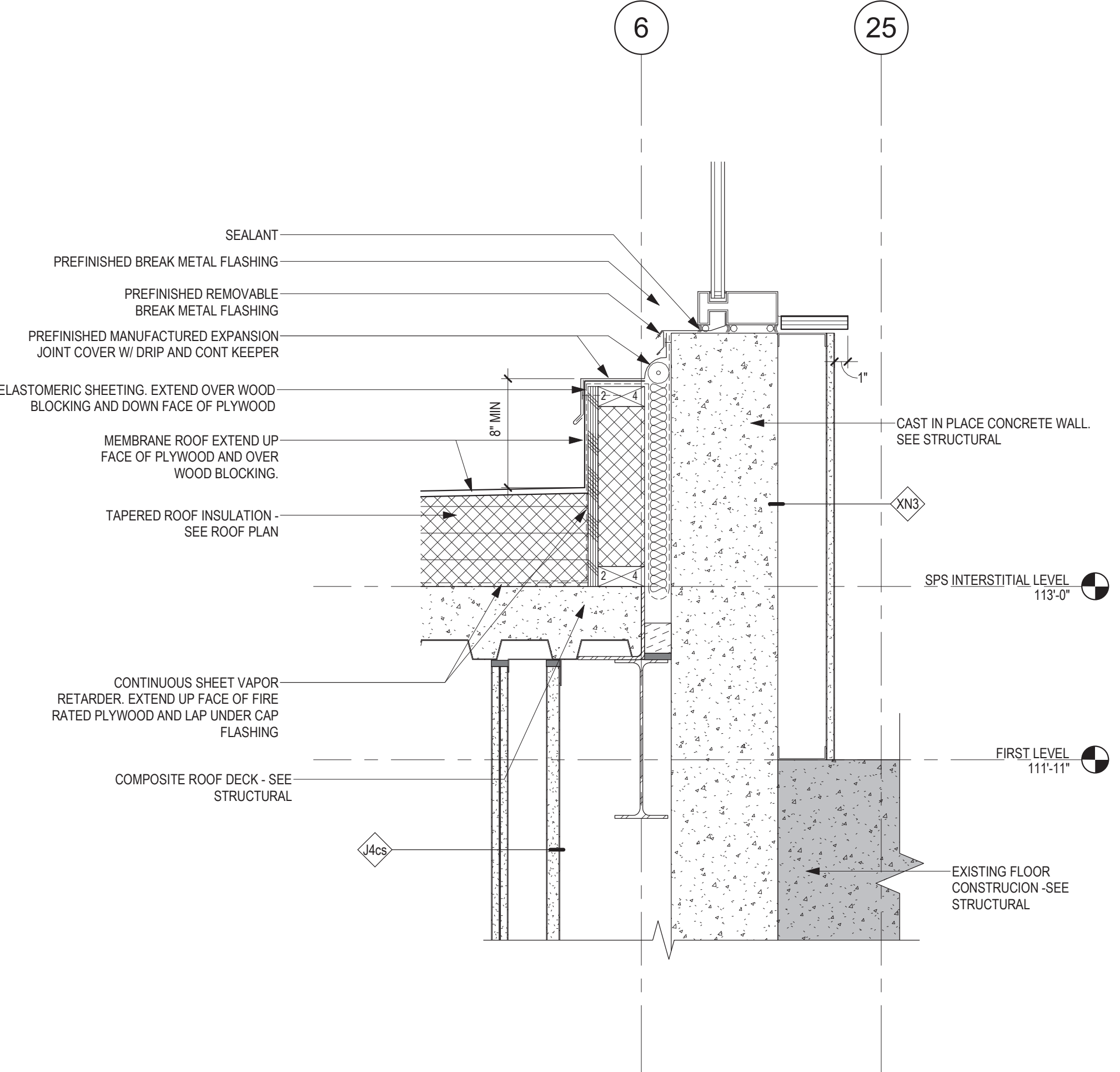
4 ROOF DETAIL - ROOF ANT MODIFIED CURTIAN WALL 1 1/2" = 1'-0"
