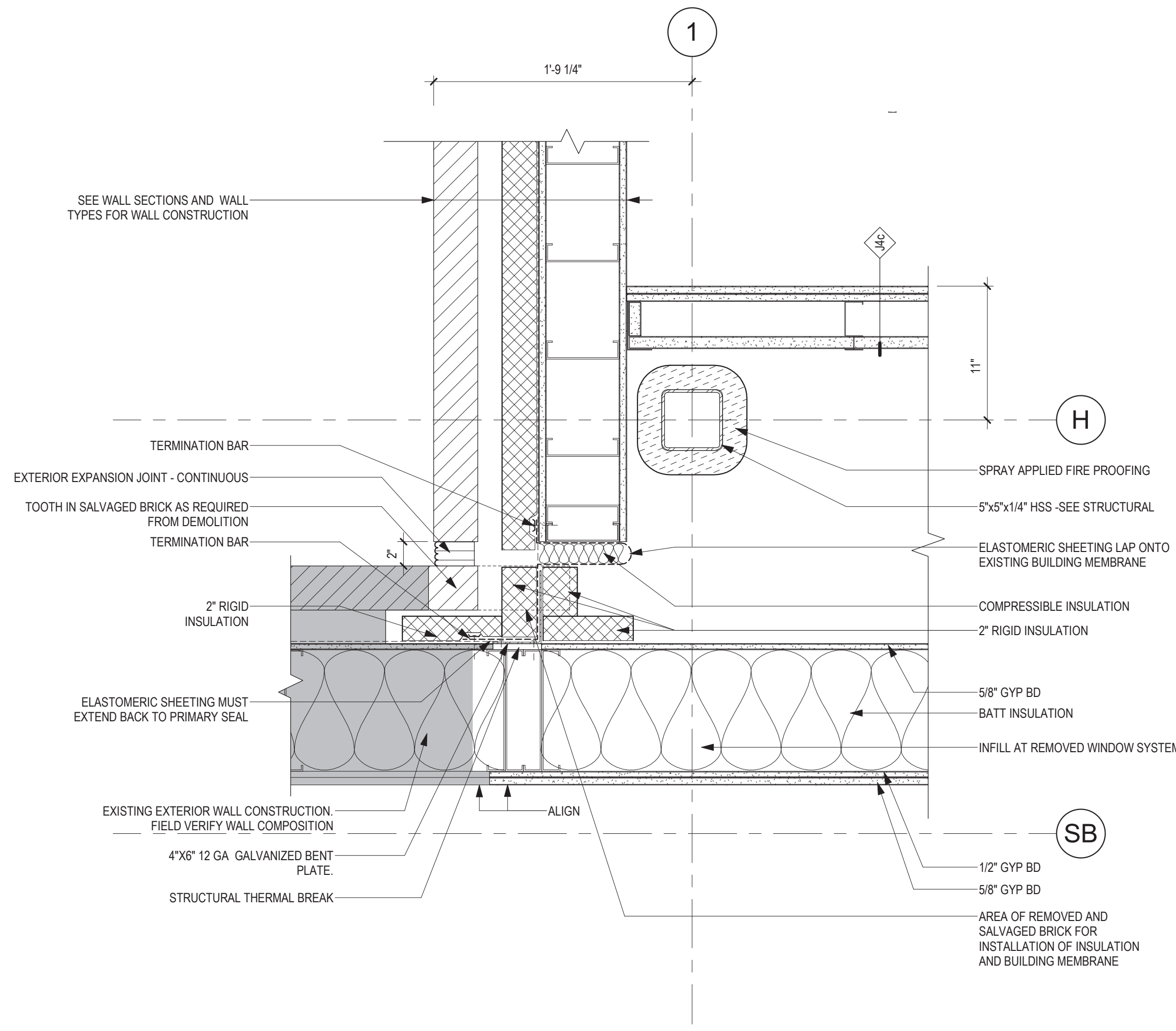
6 PLAN DETAIL -BRICK AND STEEL STUDS TO EXTING 'OPERATING SUITE' EXTERIOR WALL 1 1/2" = 1'-0"
