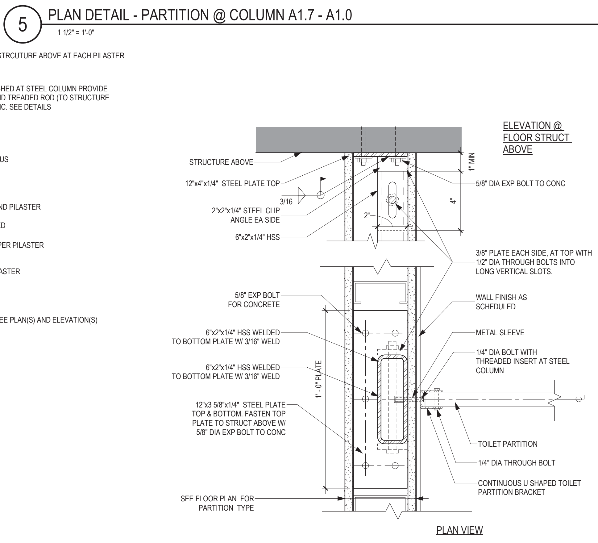
8 PLAN DETAIL - TOILET PARTITION SUPPORT 3' = 1'-0"
