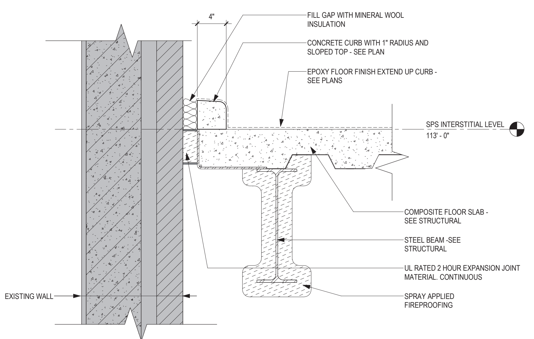
11 SECTION DETAIL - EXPANSION JOINT AT MECH ROOM (TYP) 1 1/2" = 1'-0"
