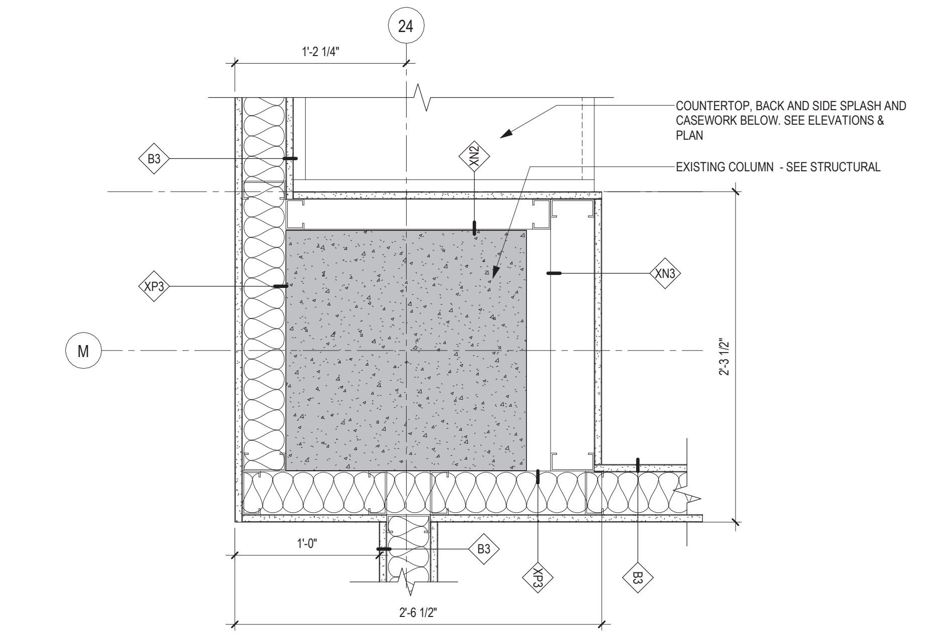
11 PLAN DETAIL - PARTITION @ COLUMN M-24 1 1/2" = 1'-0"
