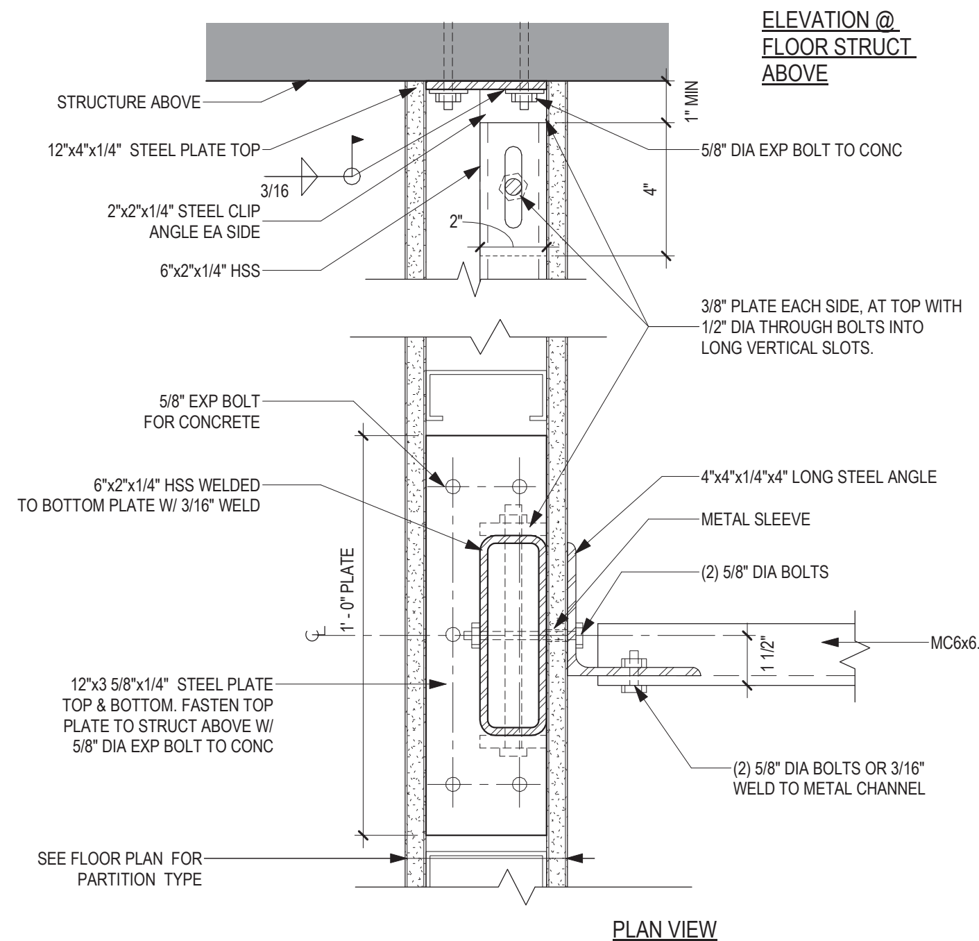
10 PLAN DETAIL - TOILET PARTITION METAL CHANNEL SUPPORT 3' = 1'-0"
