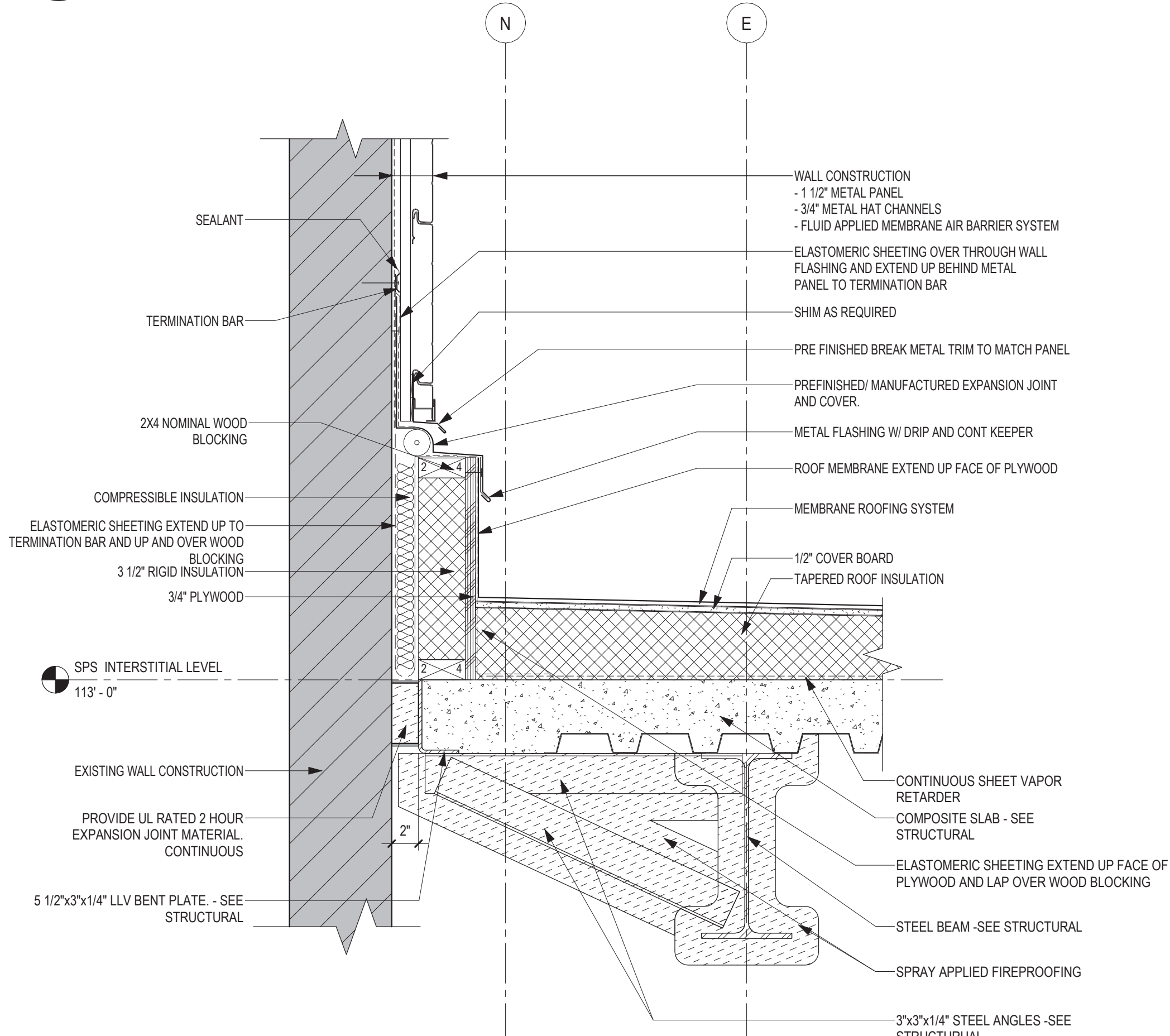
6 SECTION DETAIL - METAL PANEL BASE @ LOW ROOF GRID N 1 1/2" = 1'-0"
