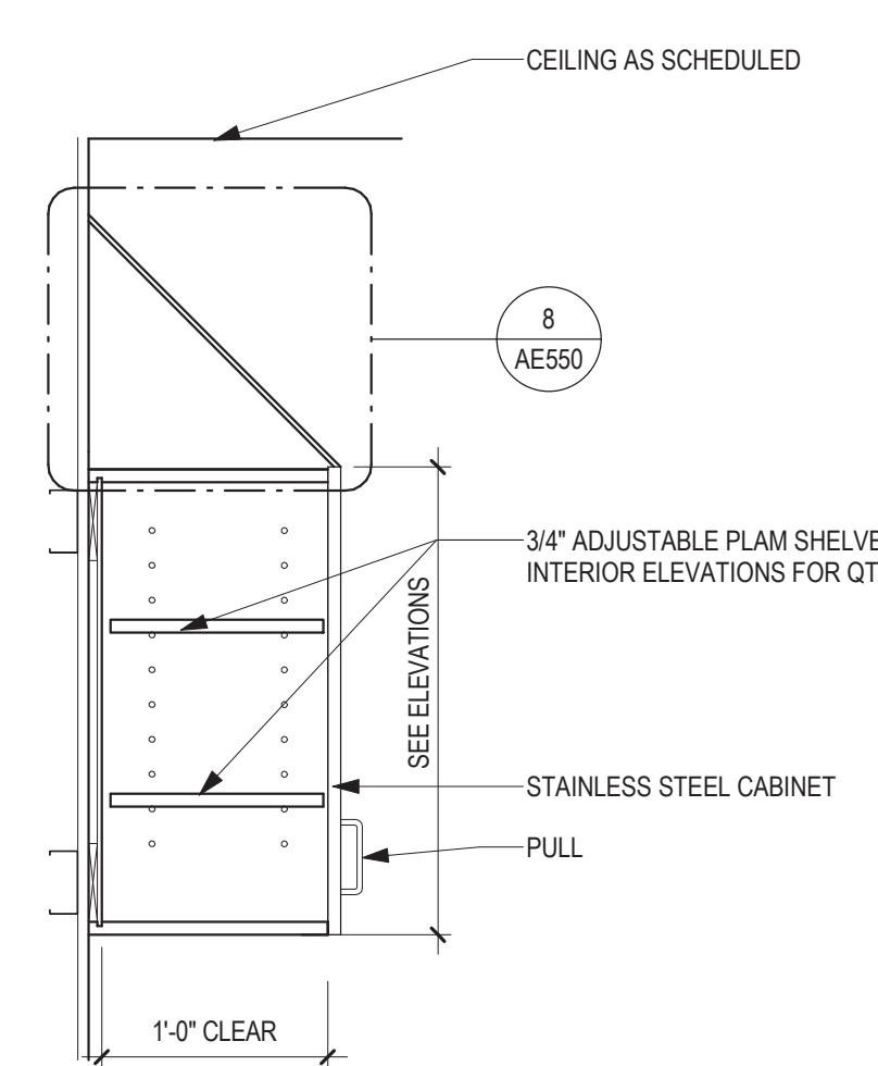
6 SECTION - STAINLESS STEEL WALL CABINET WITH DOOR 1" = 1'-0"
