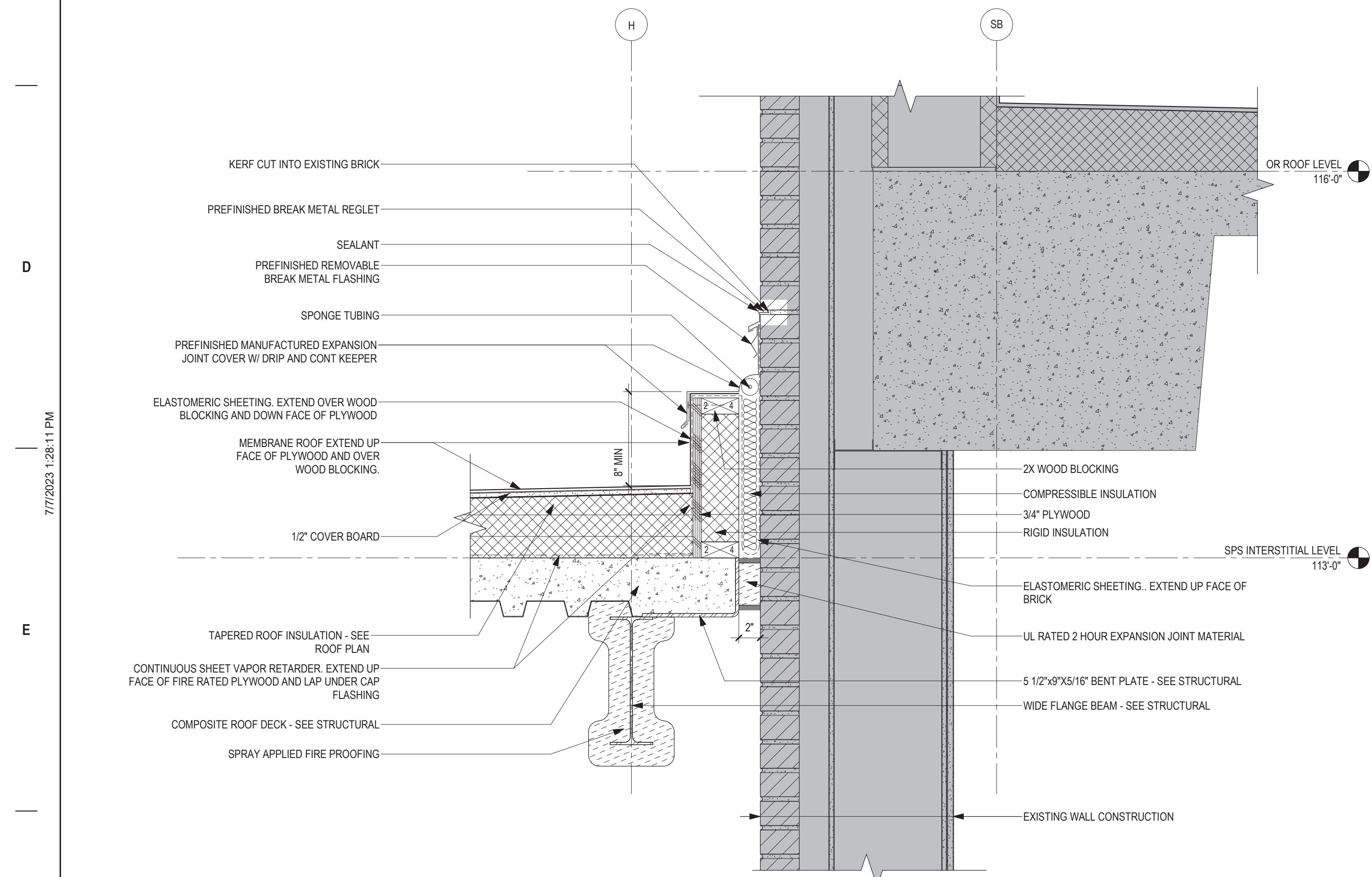
6 ROOF DETAIL - MEMBRANE ROOF @ OPERATING ROOM SUITE 1 1/2" = 1'-0"
