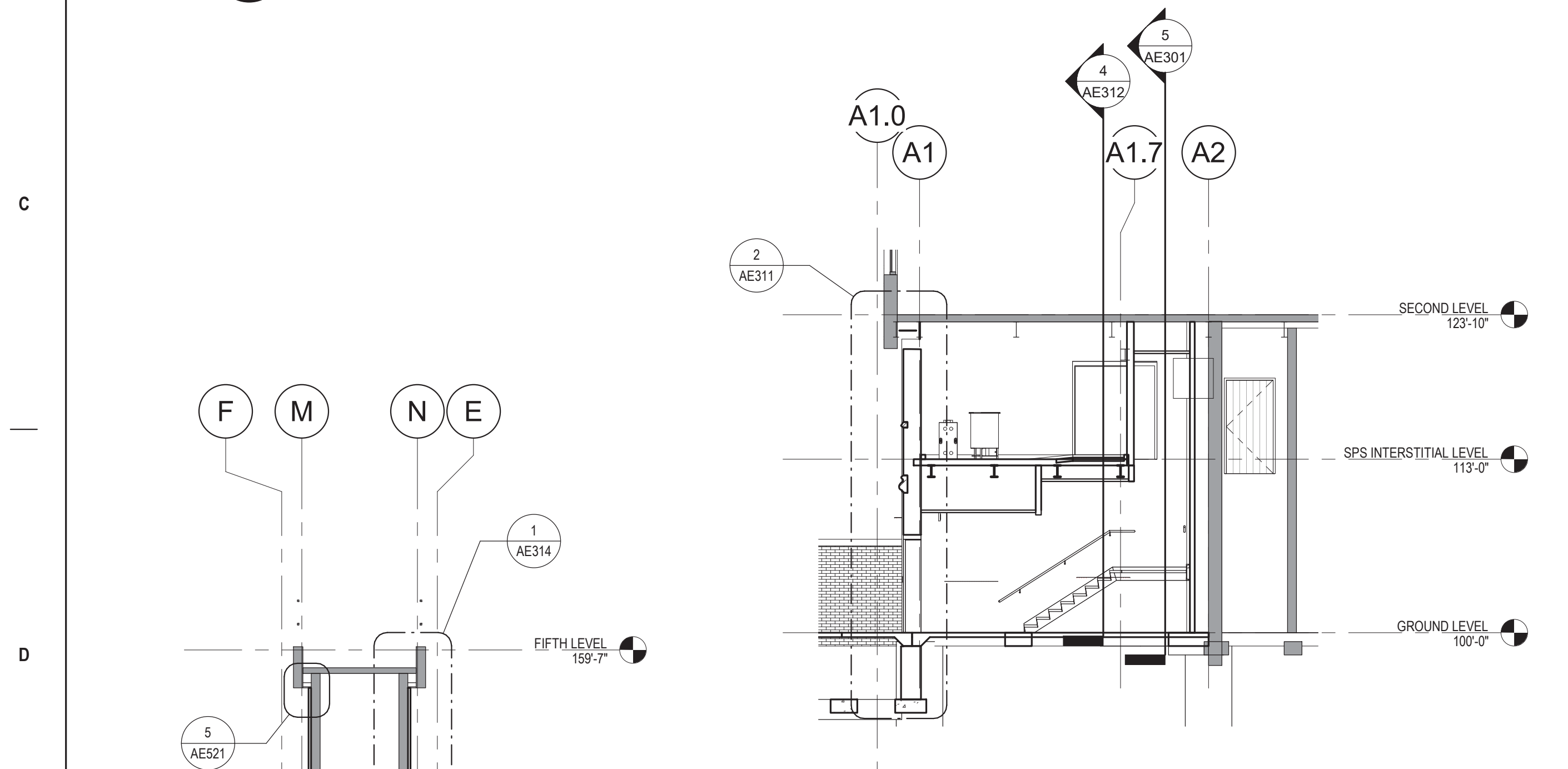
2 BUILDING SECTION - ADDITION AT EXISTING BUILDING 5 - EAST / WEST 1/8" = 1'-0"
