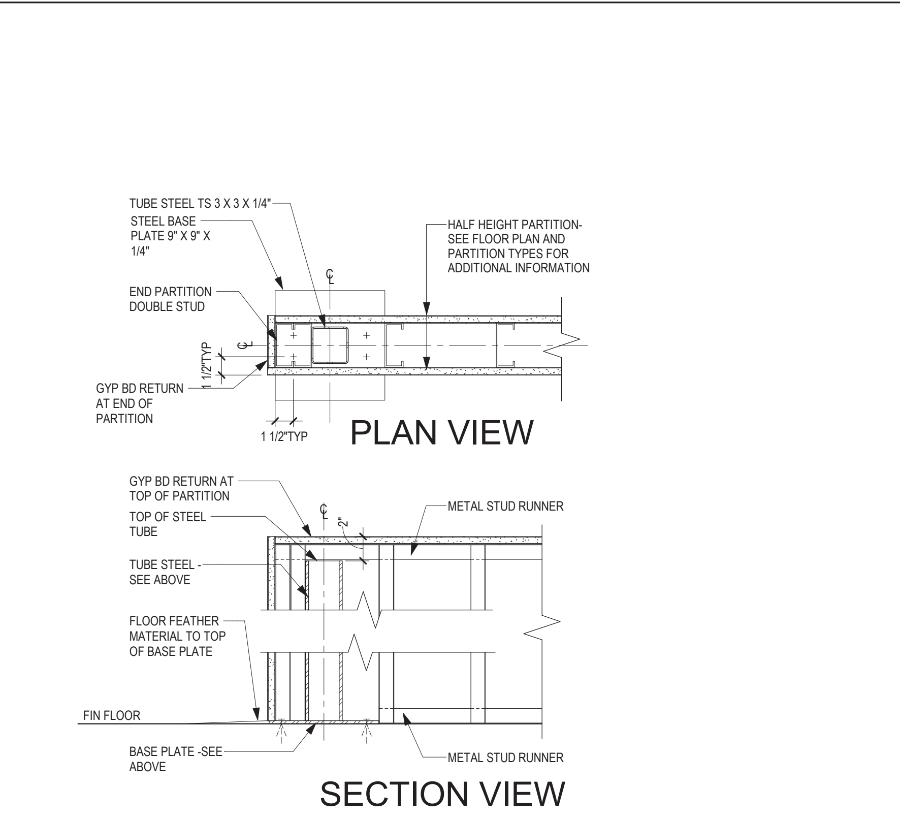
1 INTERIOR DETAIL - PARTIAL HEIGHT PARTITION-STEEL SUPPORT 1 1/2" = 1'-0"
