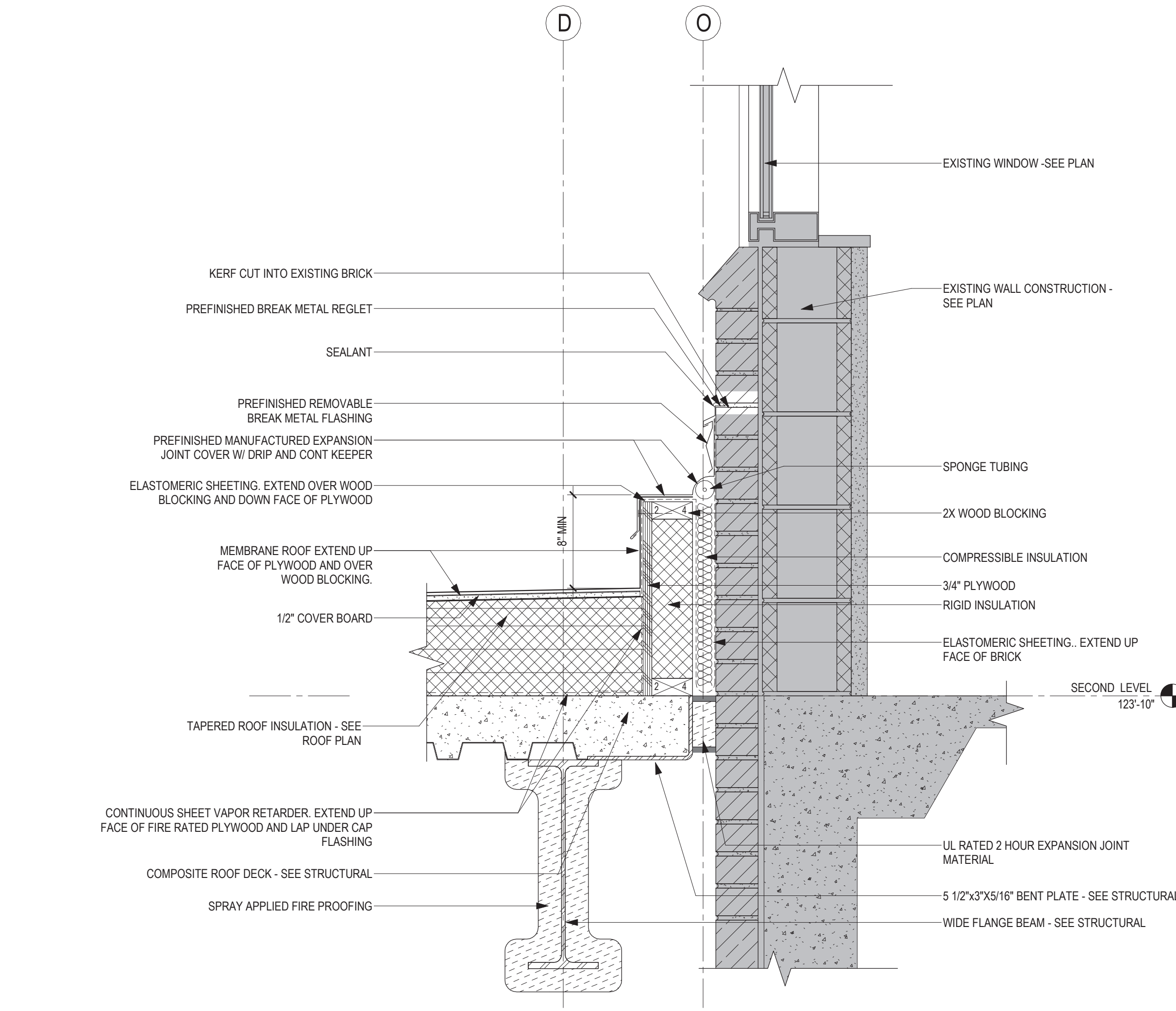
1 ROOF DETAIL - MEMBRANE ROOF @ EXISTING SECOND LEVEL WINDOW 1 1/2" = 1'-0"
