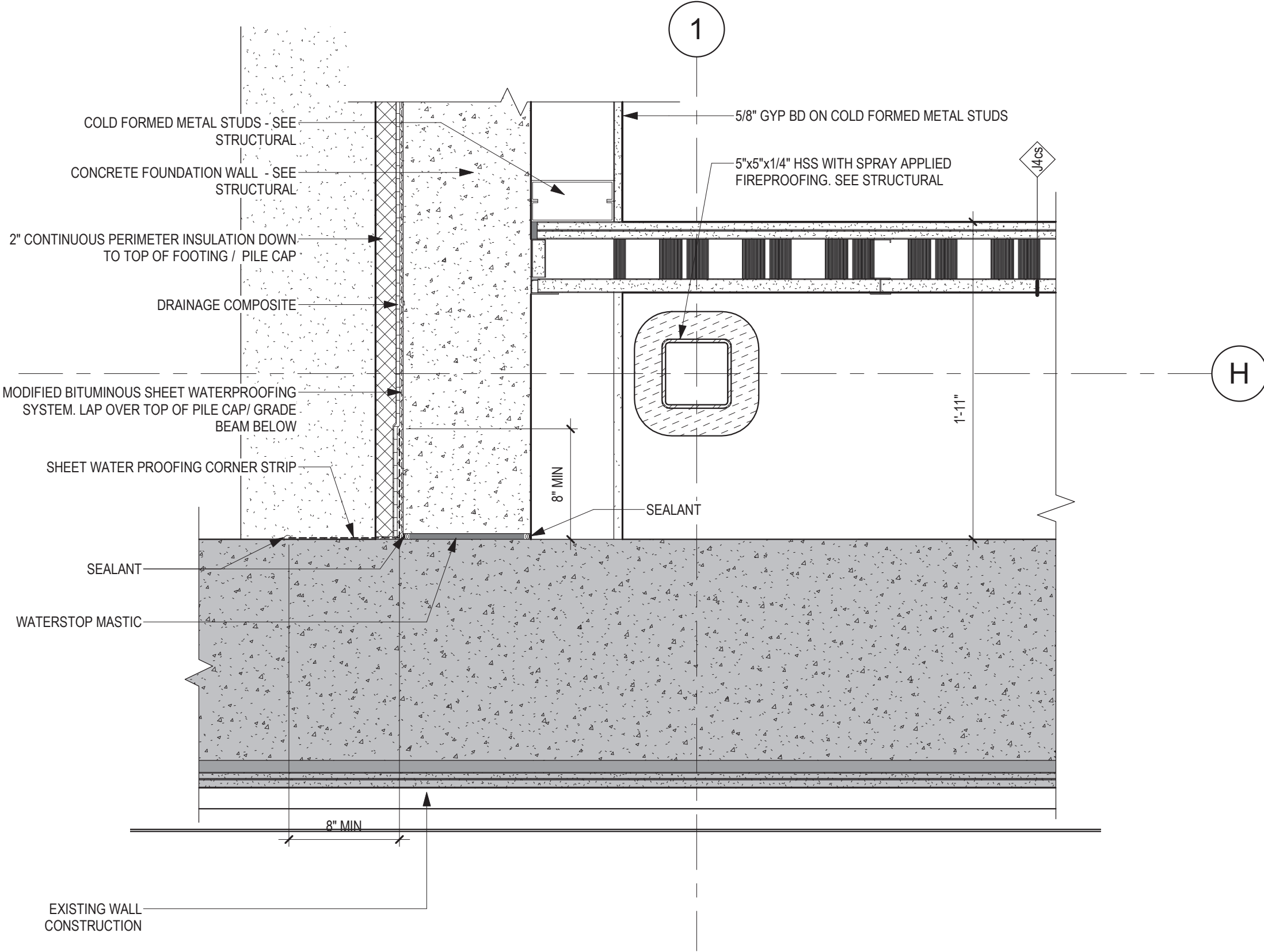
3 PLAN DETAIL - CAST IN PLACE CONCRETE TO EXTING OR EXTERIOR WALL 1 1/2" = 1'-0"
