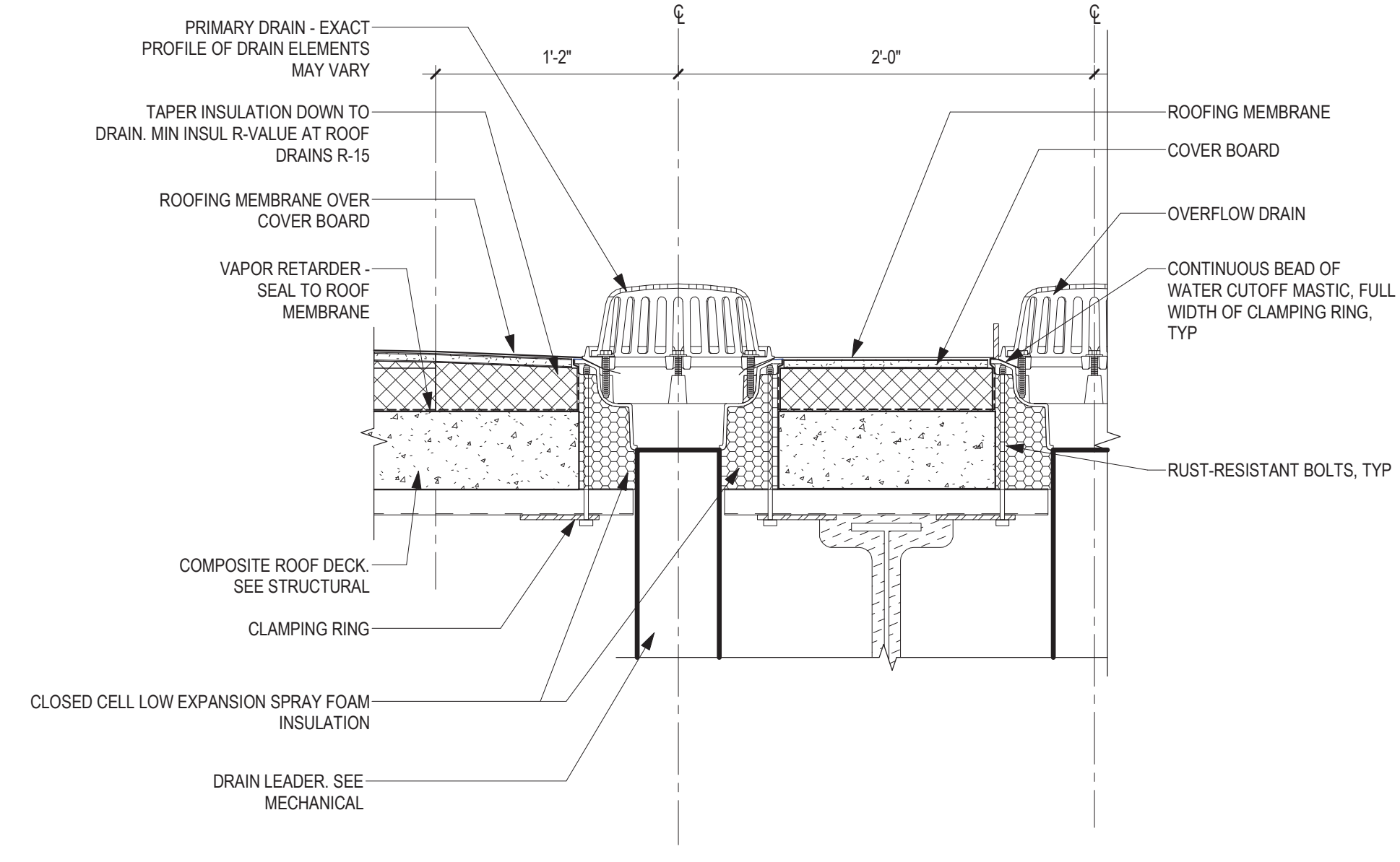
1 SECTION DETAIL - ROOF DRAINS 1 1/2" = 1'-0"
