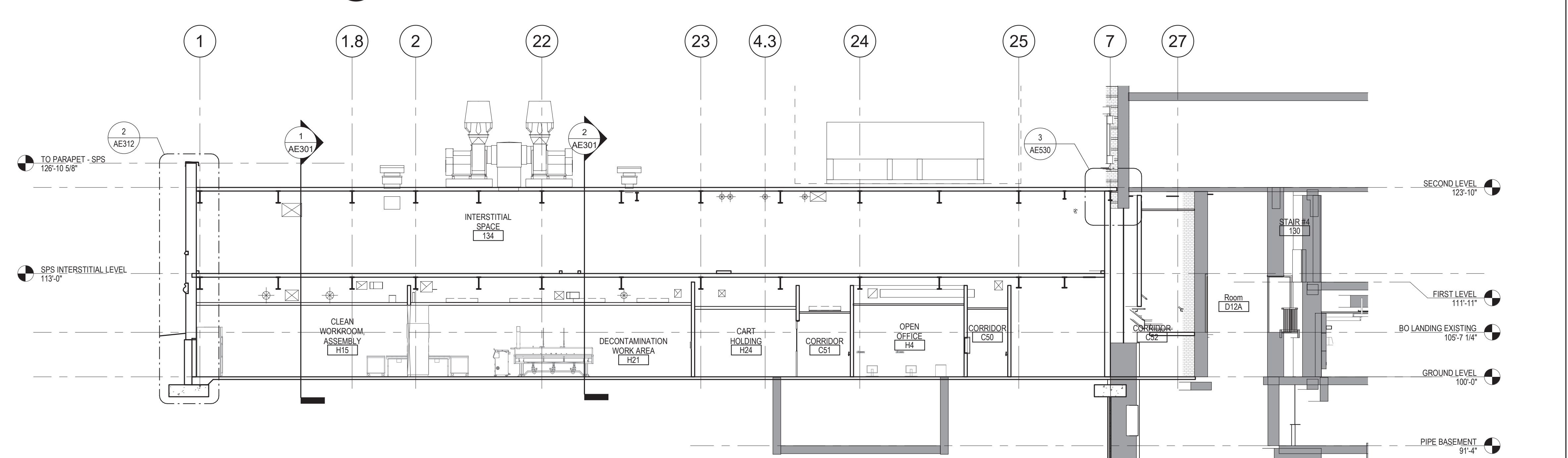
1 BUILDING SECTION - ADDITION AT EXISTING STAIR TOWER - EAST / WEST 1/8" = 1'-0"
