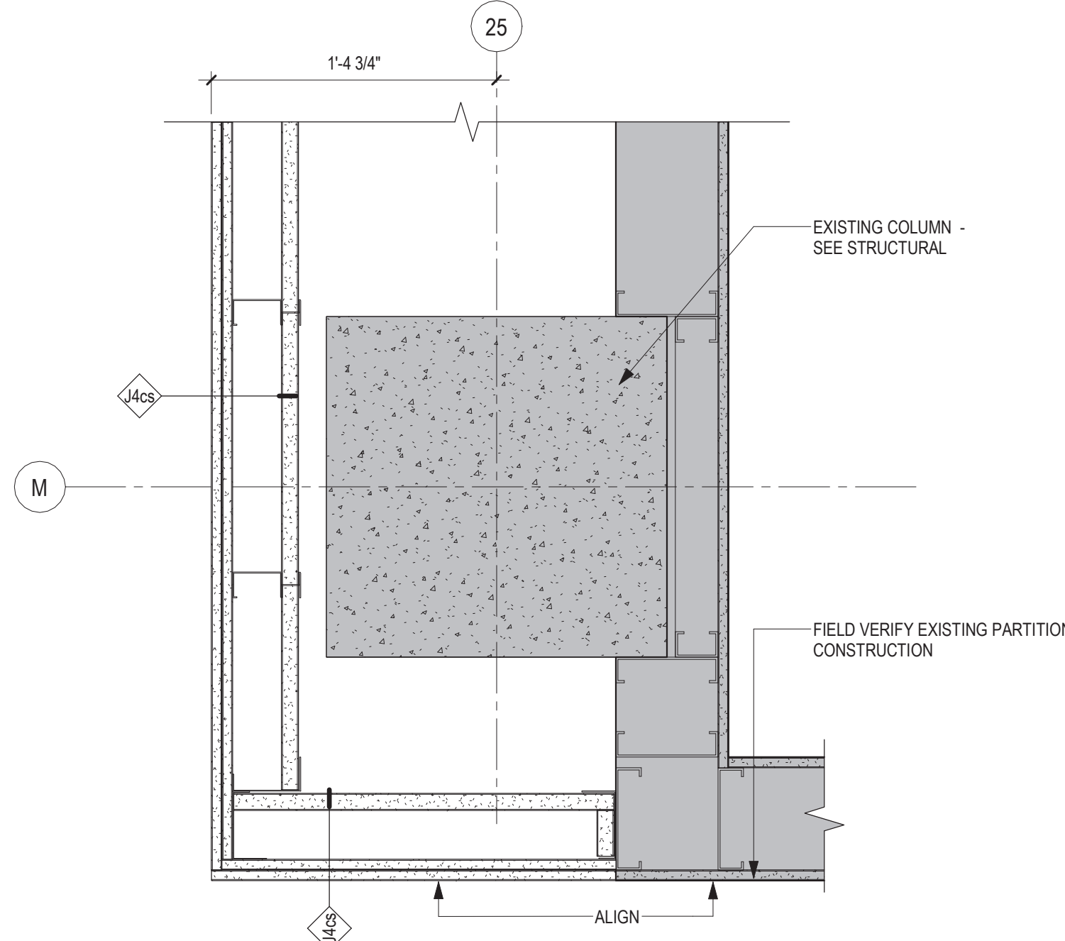
3 PLAN DETAIL - PARTITION @ COLUMN M-25 1 1/2" = 1'-0"
