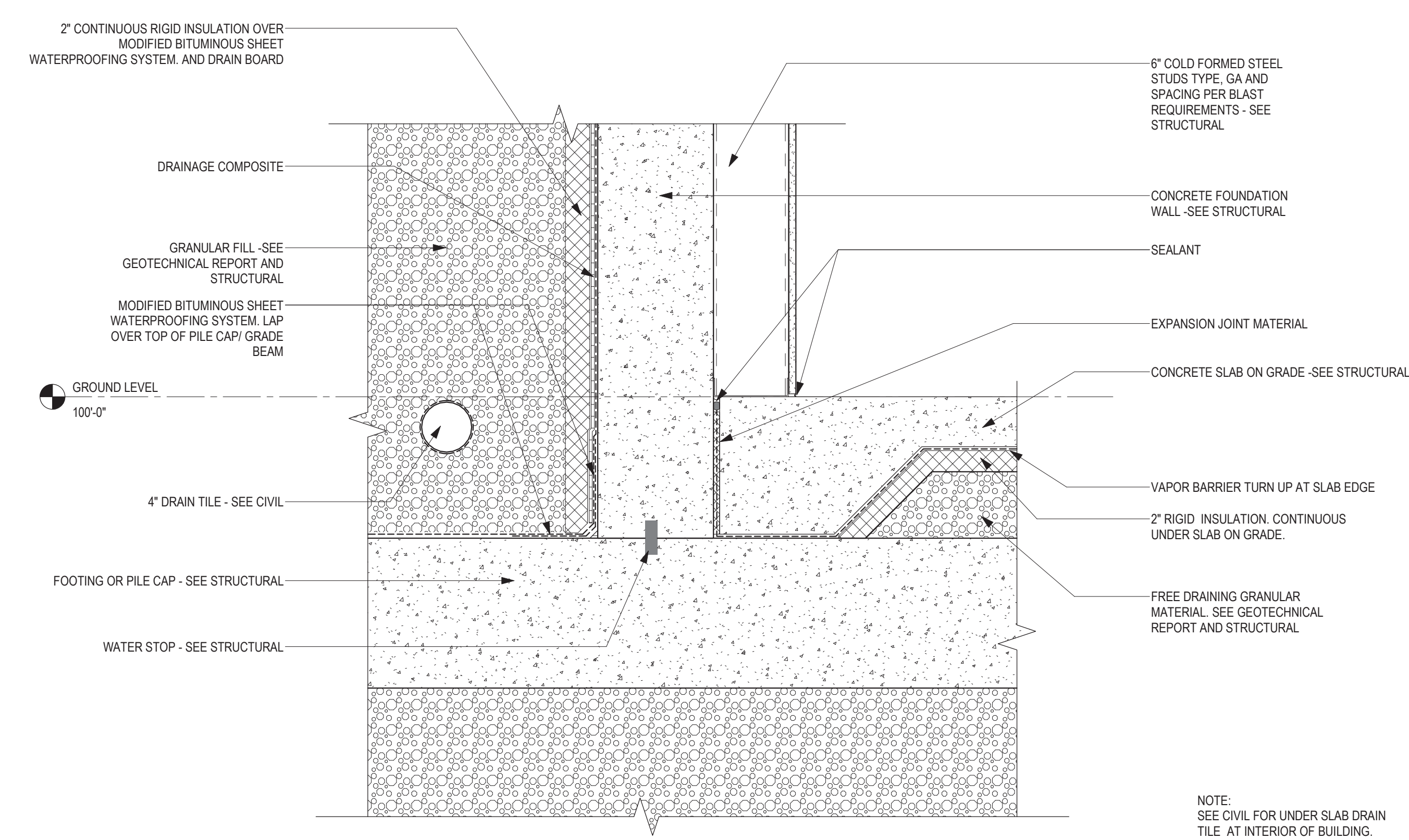
7 SECTION DETAIL - GRADE BEAM / PILE CAP AND FOUNDATION WALL WATERPROOFING (TYP) 1 1/2" = 1'-0"
