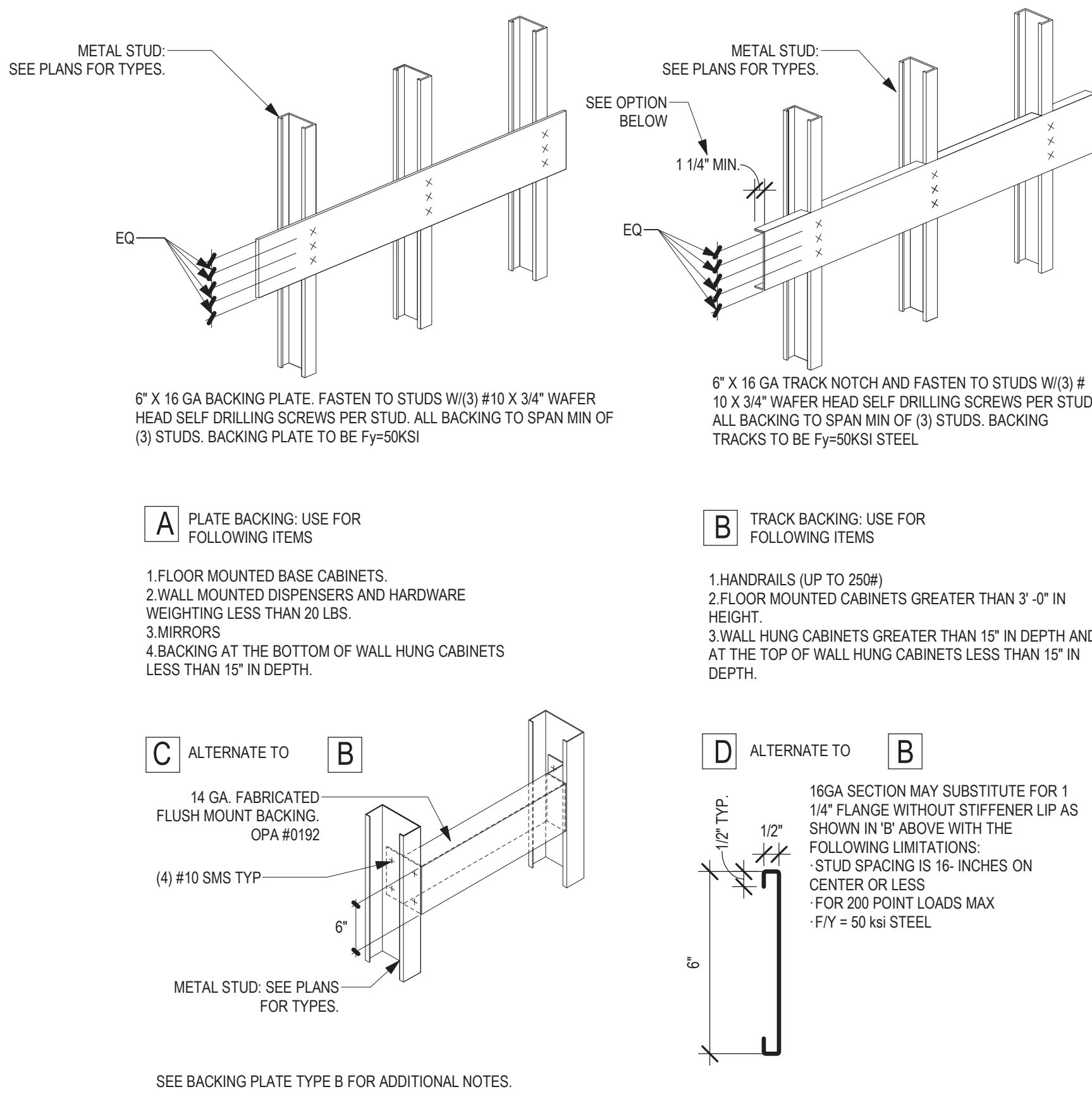
PARTITION BLOCKING-BACKING TYPES
