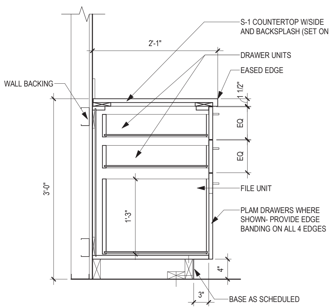
5 SECTION - BASE CABINET 3 DRAWER W/ 2 EQ 1" = 1'-0"
