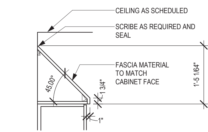
8 CASEWORK UPPER WITH SLOPED TOP 3/4" = 1'-0"
