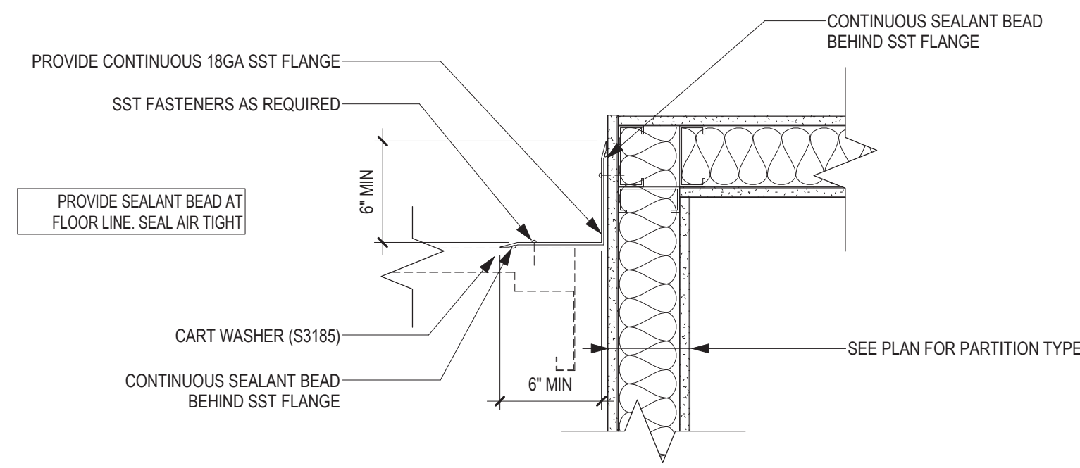
2 PLAN DETAIL - SST BARRIER FLANGE @ CART WASH 1 1/2" = 1'-0"
