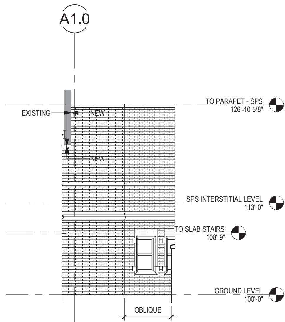
4 PARTIAL EXTERIOR ELEVATION - NORTH 1/8" = 1'-0"
