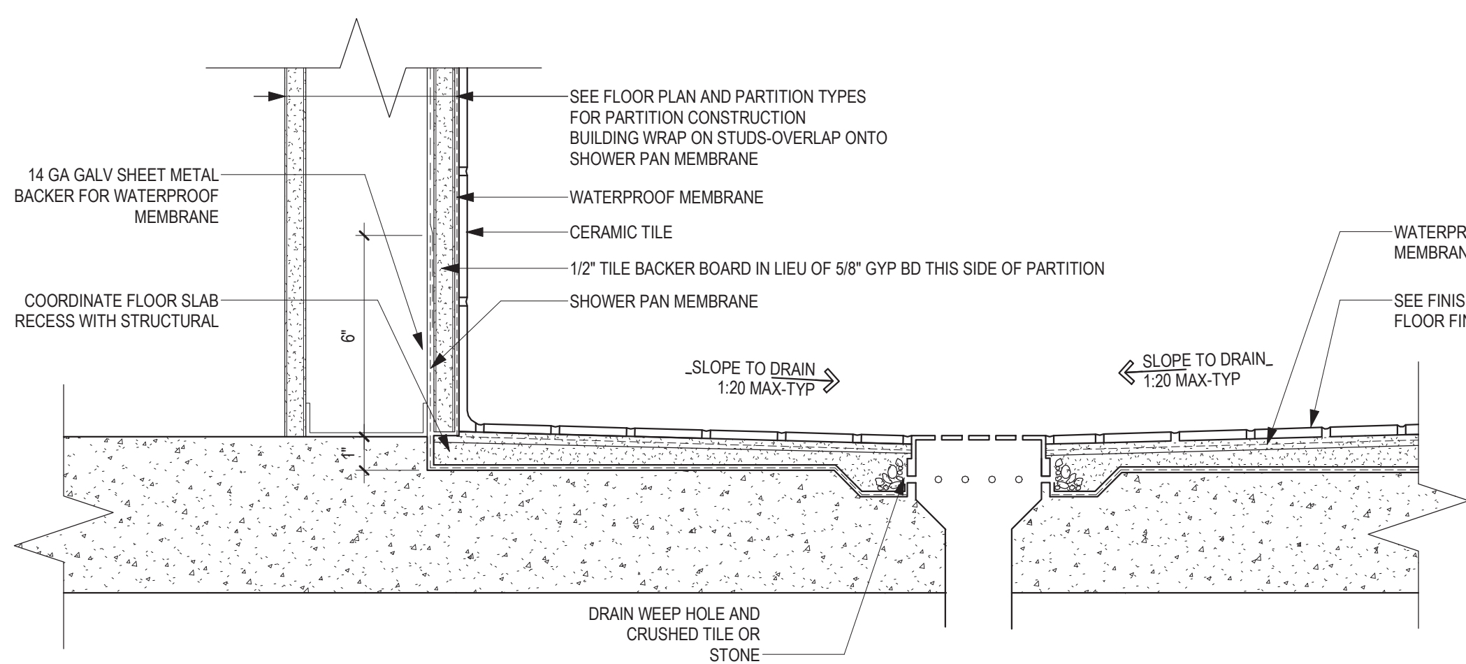
10 SECTION DETAIL INTERIOR - WATERPROOFING AT TOILET ROOM FLOOR 3" = 1'-0"
