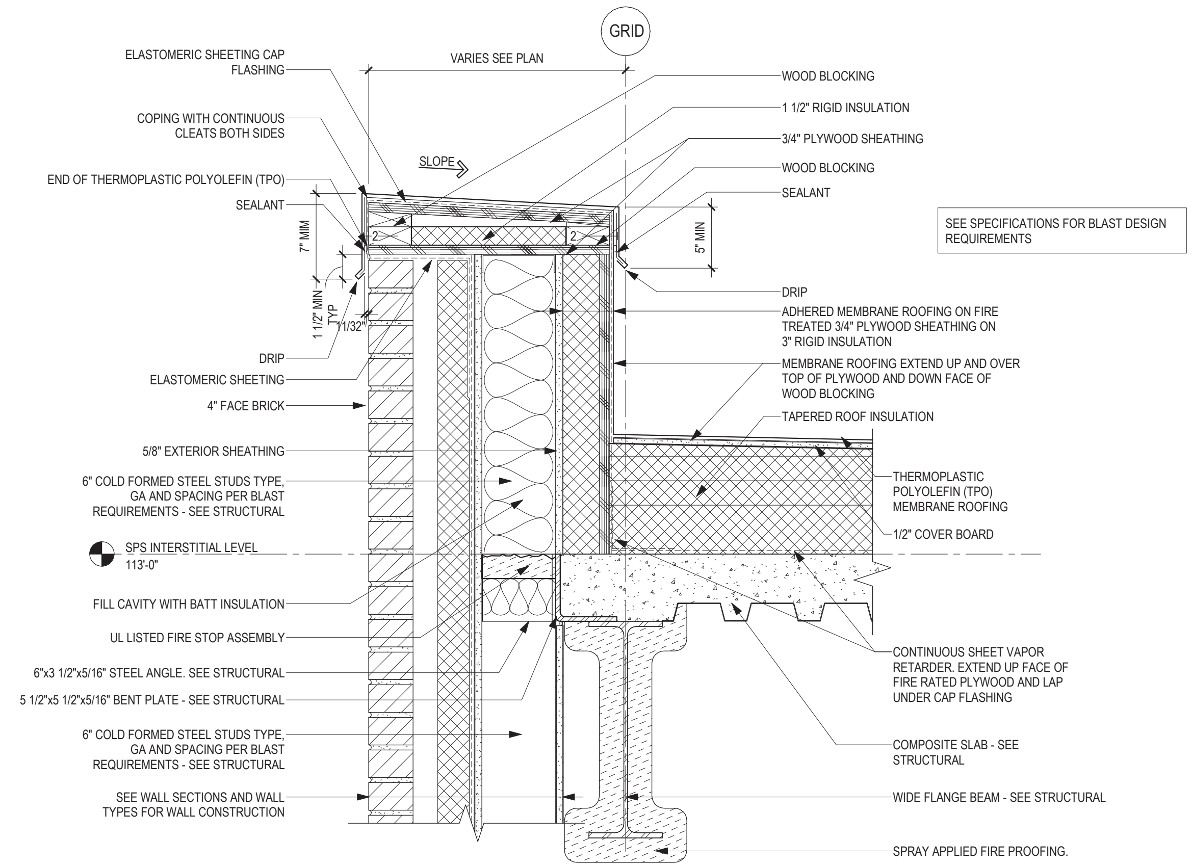
1 SECTION DETAIL - PARAPET AT BRICK WALL WITH METALS STUD BACK UP 1 1/2" = 1'-0"
