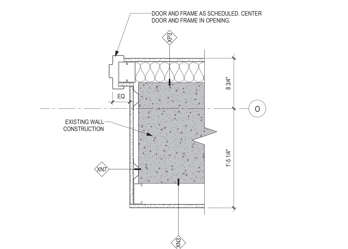
8 PLAN DETAIL - PARTITION AND DOOR JAMB AT DOOR H20AA 1 1/2" = 1'-0"
