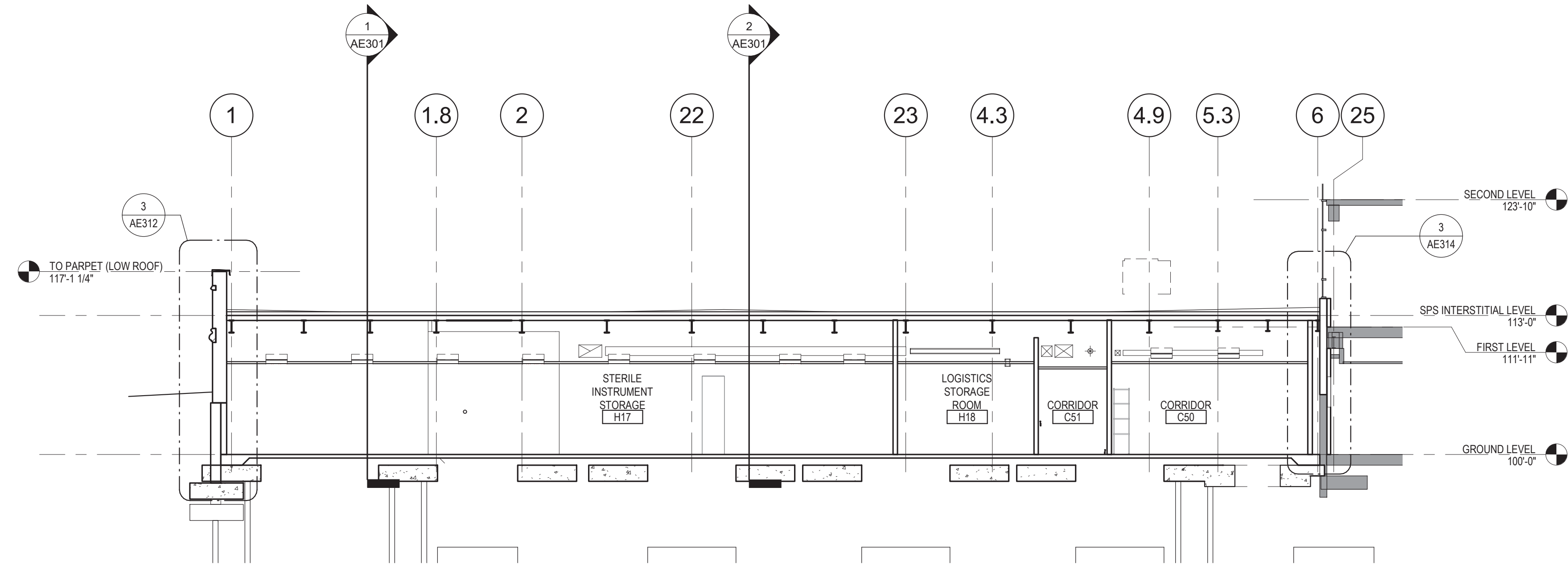
2 BUILDING SECTION - SINGLE STORY ADDITON @ ELEVATOR TOWER LINK - NORTH / SOUTH 1/8" = 1'-0"
