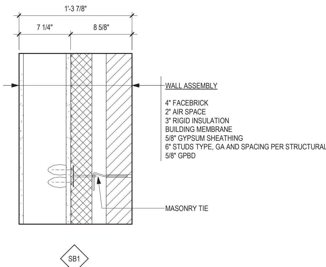
TYPES - WALL
