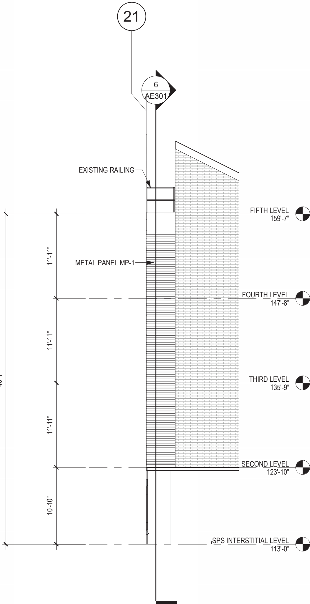
6 EXTERIOR ELEVATION - STAIR TOWER - WEST 1/8" = 1'-0"
