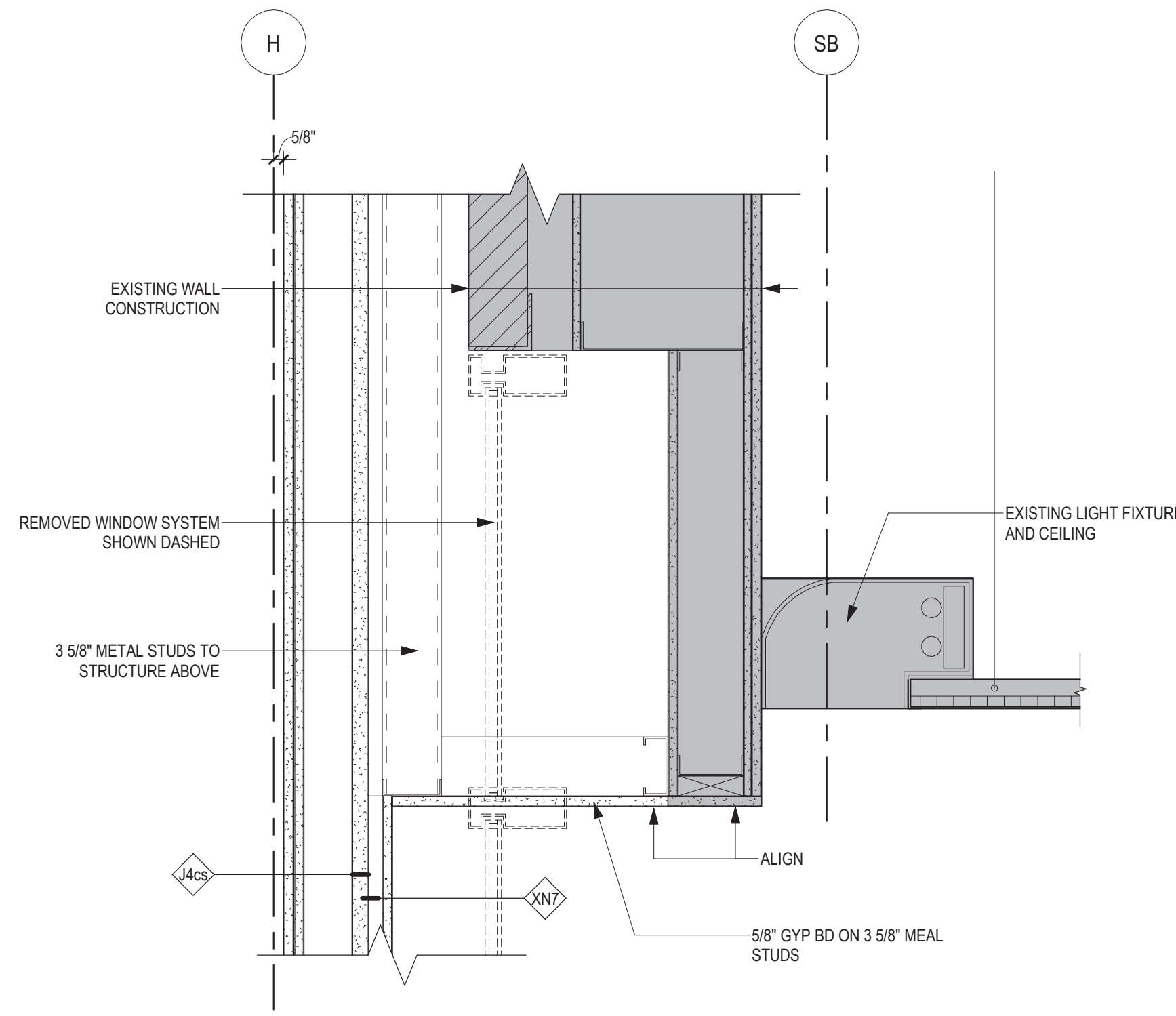
12 SECTION DETAIL - OPENING AT SURGERY / OR CORRIDOR 1 1/2" = 1'-0"
