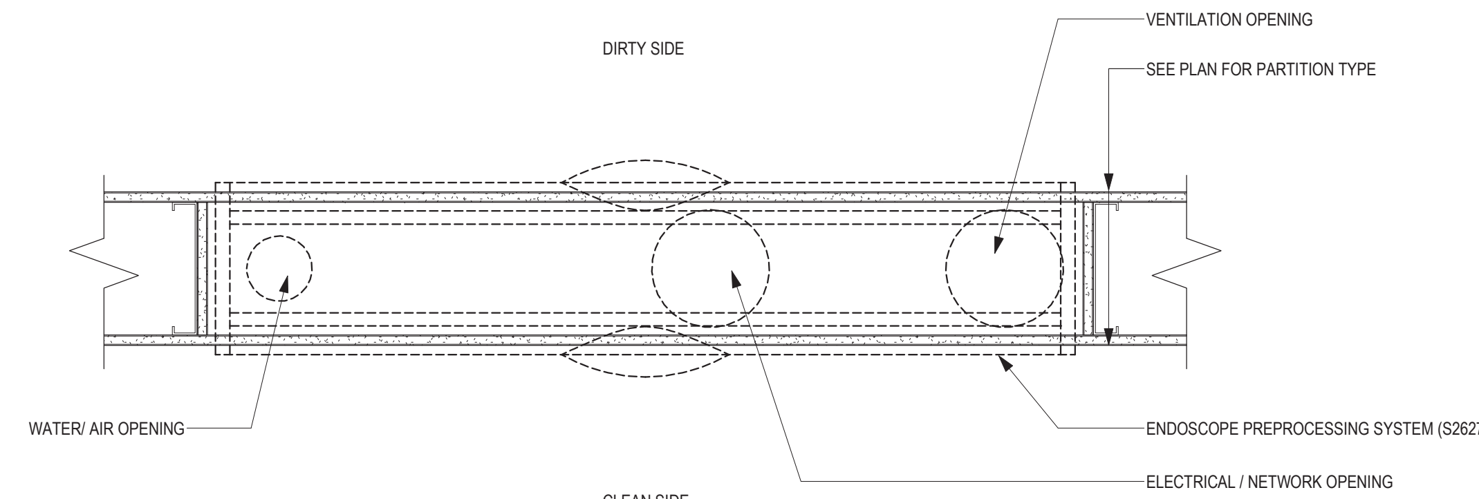
4 PLAN DETAIL - PARTITION @ COLUMN A1.7 - 30.4 1 1/2" = 1'-0"
