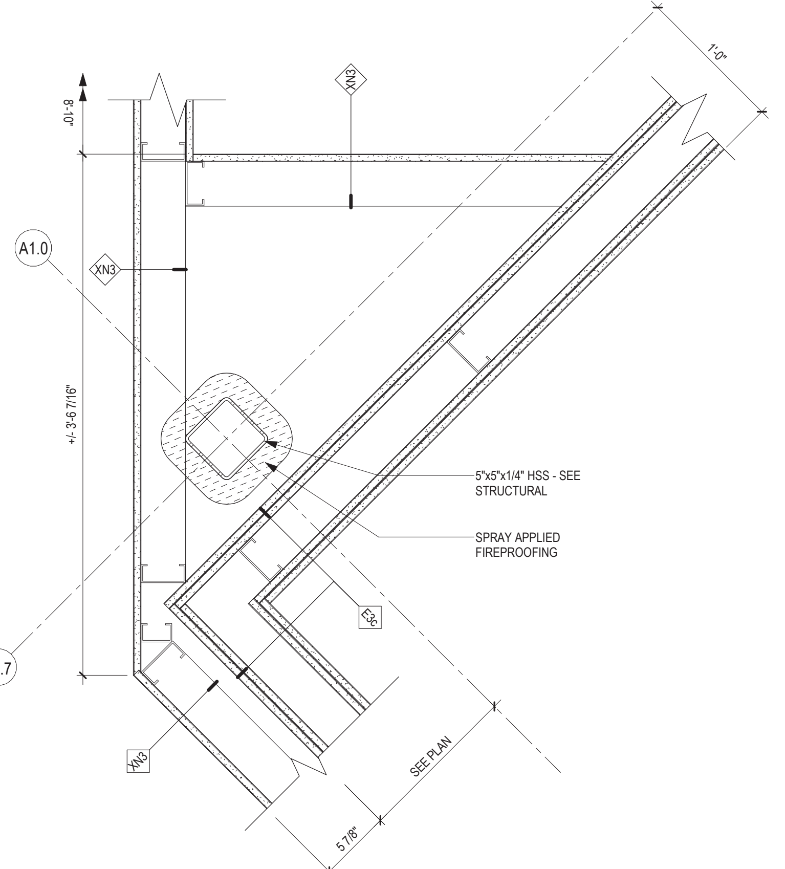
5 PLAN DETAIL - PARTITION @ COLUMN A1.7 - A1.0 1 1/2" = 1'-0"
