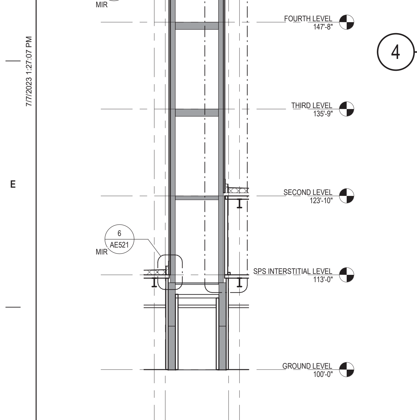
6 SECTION - EXISTING STAIR TOWER - EAST/WEST 1/8" = 1'-0"
