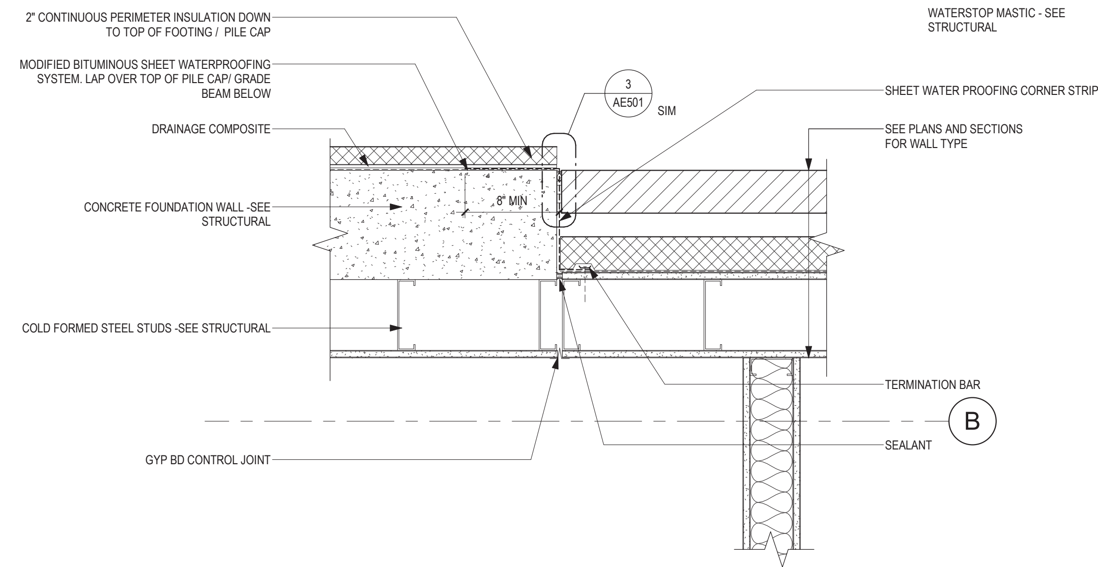
1 PLAN DETAIL - BRICK AND STEEL STUD TO CAST IN PLACE CONCRETE TRANSITION 1 1/2" = 1'-0"
