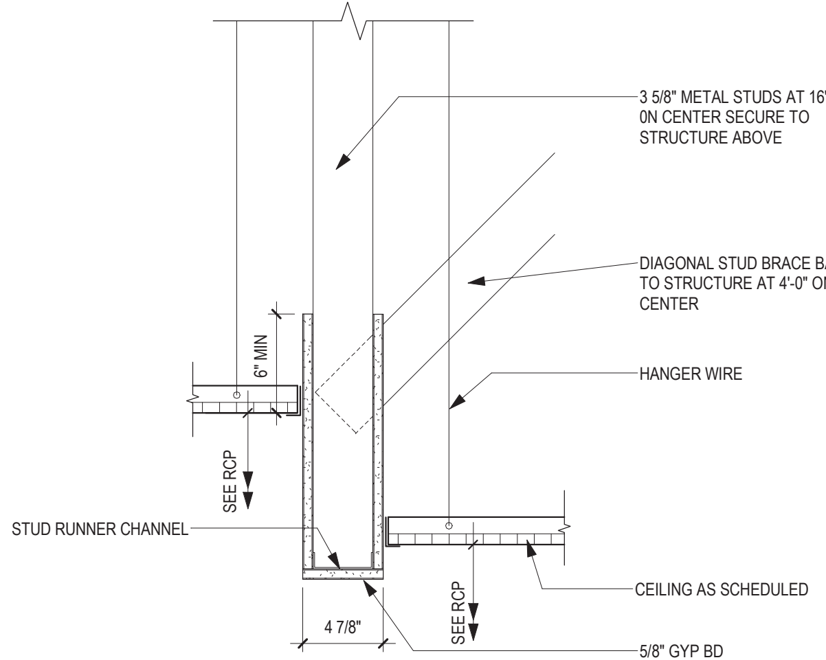
SECTION DETAIL - GYP BD BULKHEAD 1 1/2" = 1'-0"
