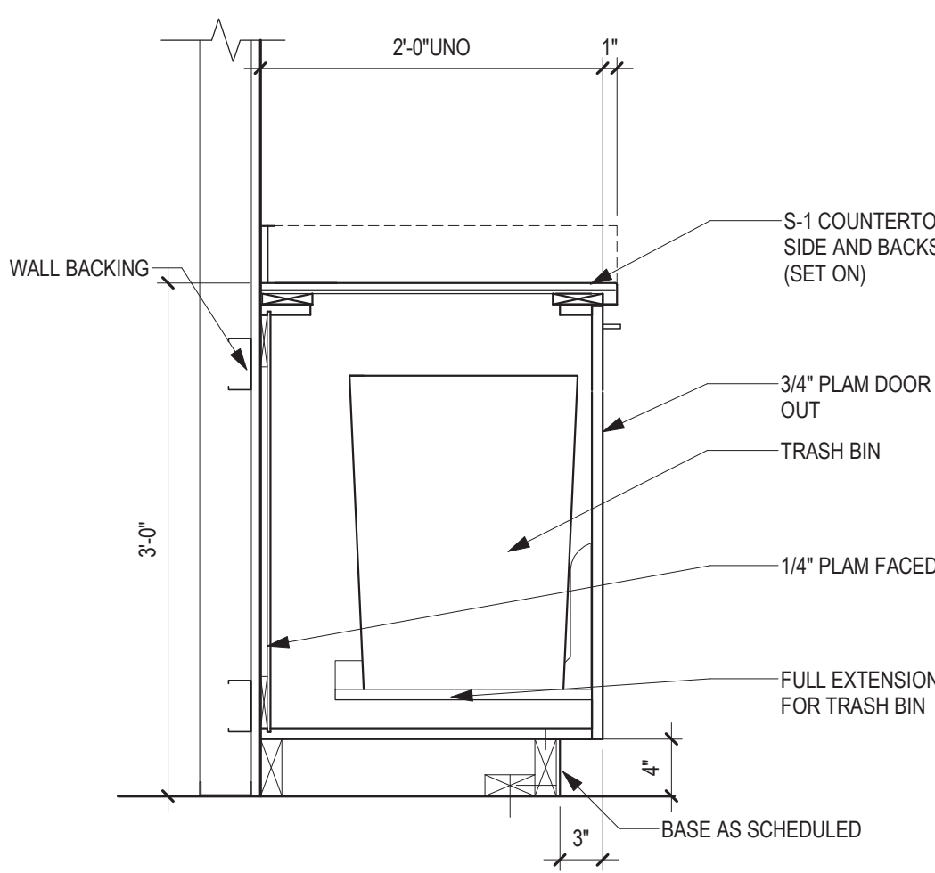
4 SECTION - BASE CABINET TRASH 1" = 1'-0"
