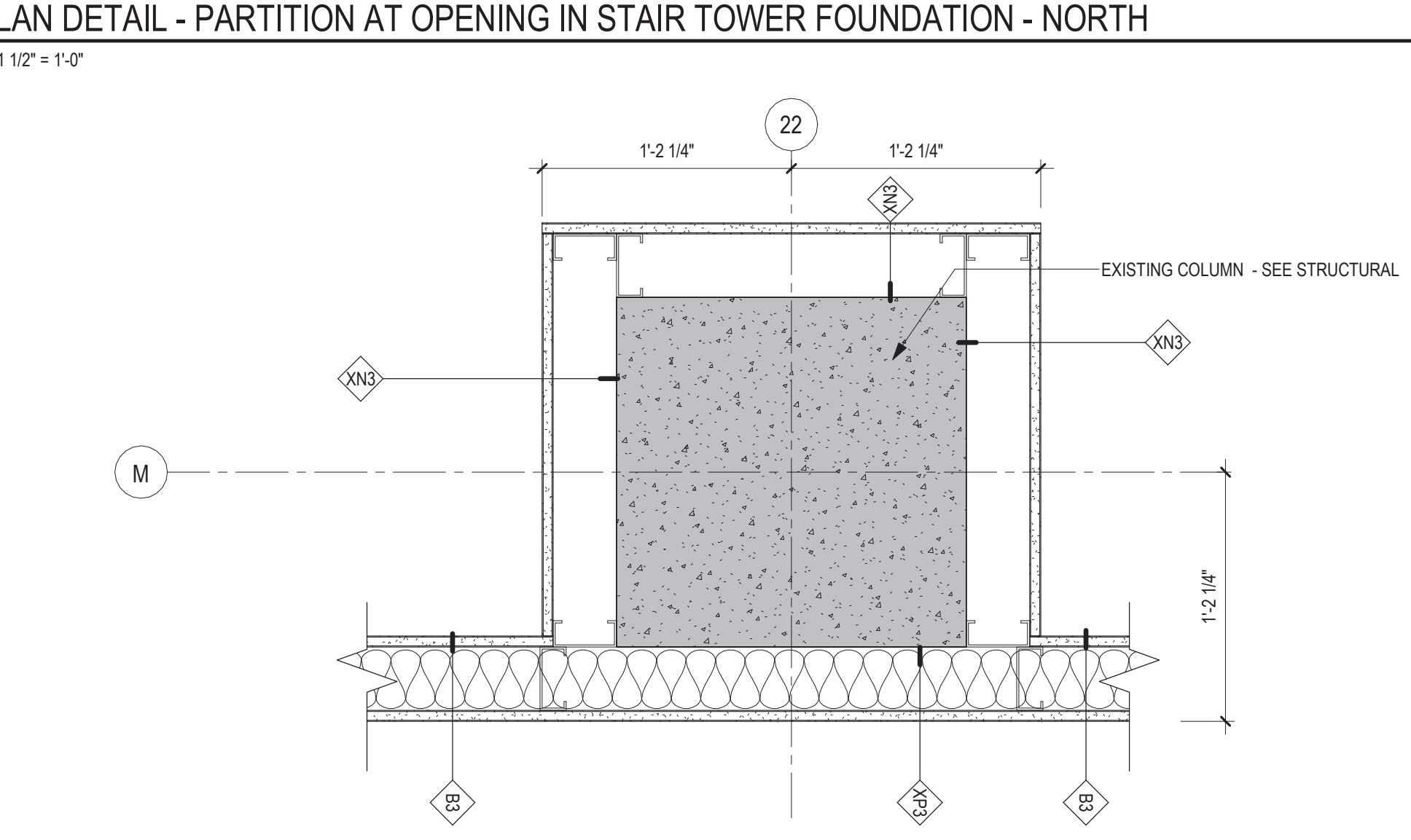
9 PLAN DETAIL - PARTITION @ COLUMN M-22 1 1/2" = 1'-0"
