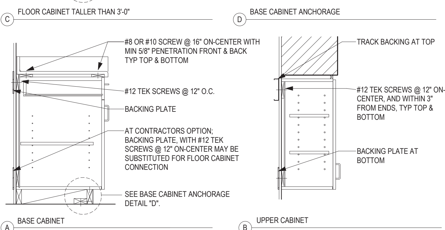
9 CASEWORK ANCHORAGE 3/4" = 1'-0"
