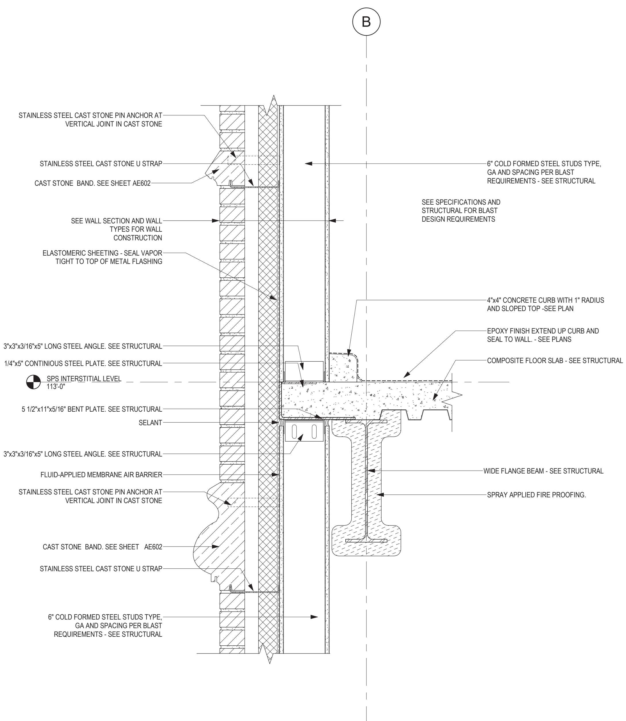
1 SECTION DETAIL - STONE BAND & SLAB EDGE 1 1/2" = 1'-0"
