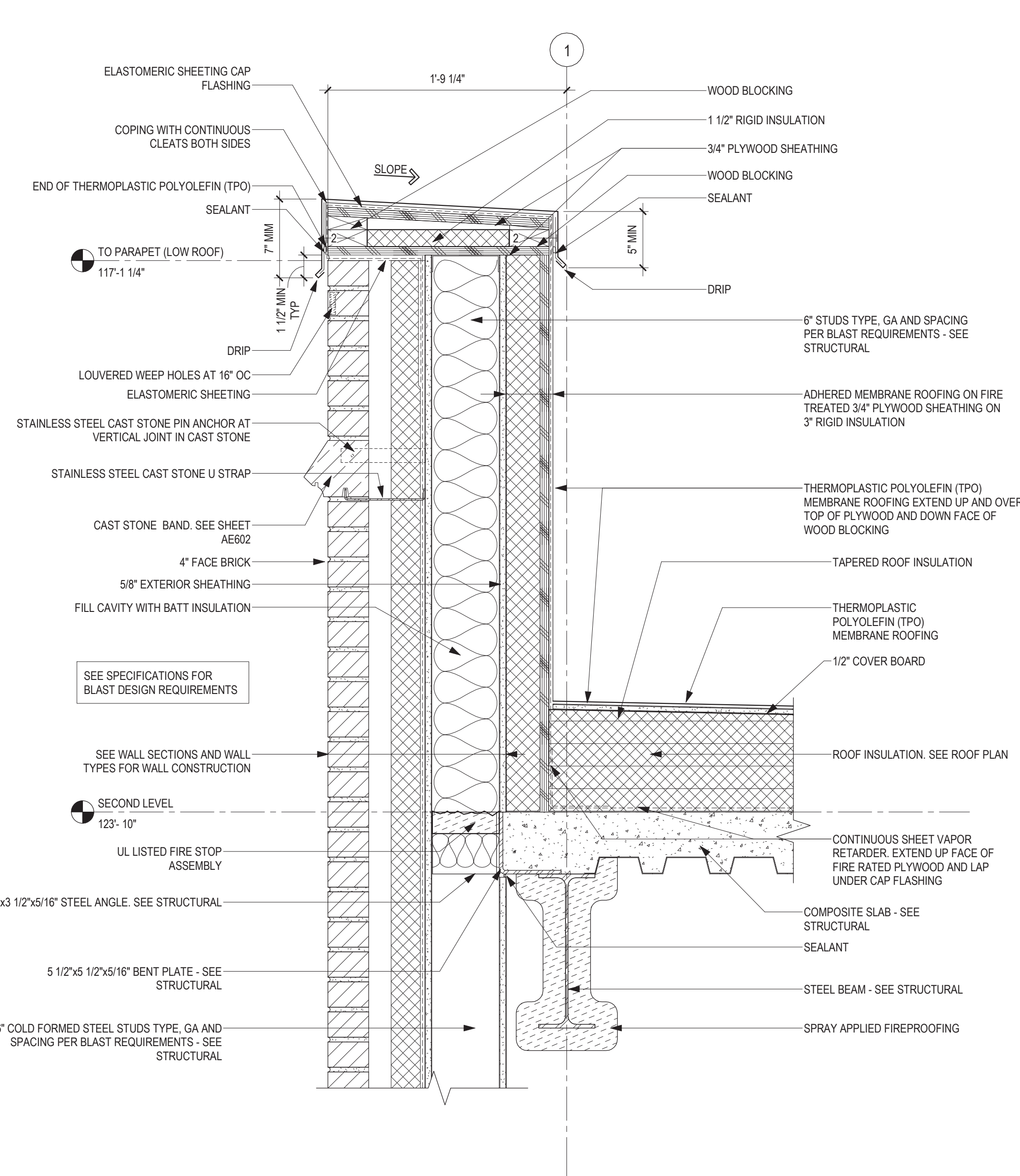
2 SECTION DETAIL - PARAPET AT BRICK WALL WITH METALS STUD - LOW ROOF 1 1/2" = 1'-0"
