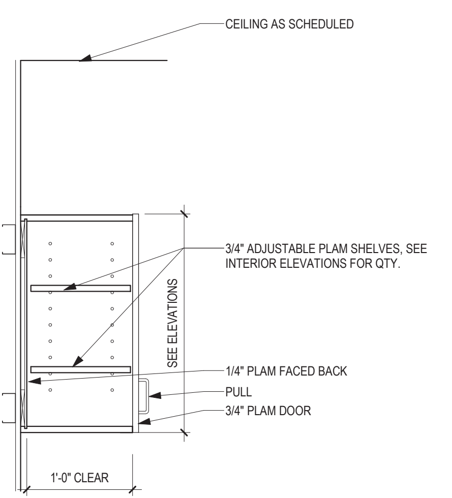
1 SECTION - WALL CABINET WITH DOOR 1" = 1'-0"
