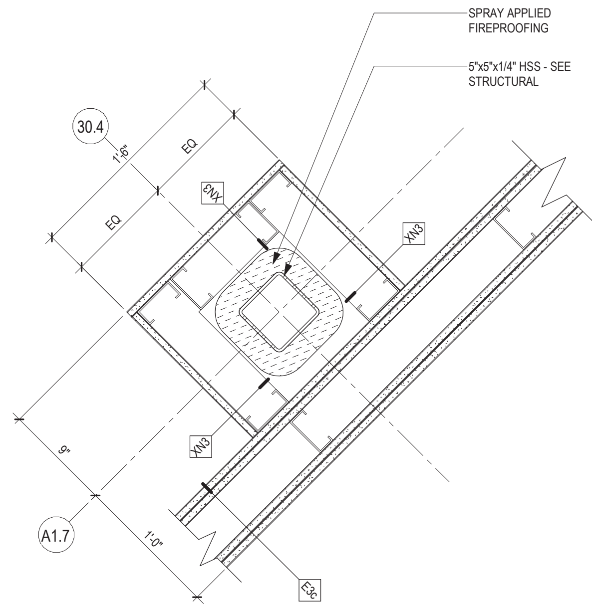
4 PLAN DETAIL - PARTITION @ COLUMN A1.7 - 30.4 1 1/2" = 1'-0"
