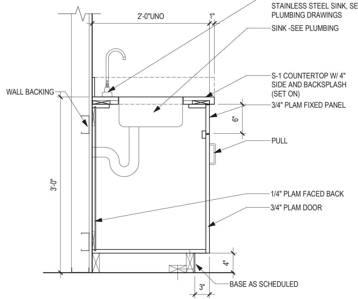
3 SECTION - BASE CABINET WITH SINK 1" = 1'-0"
