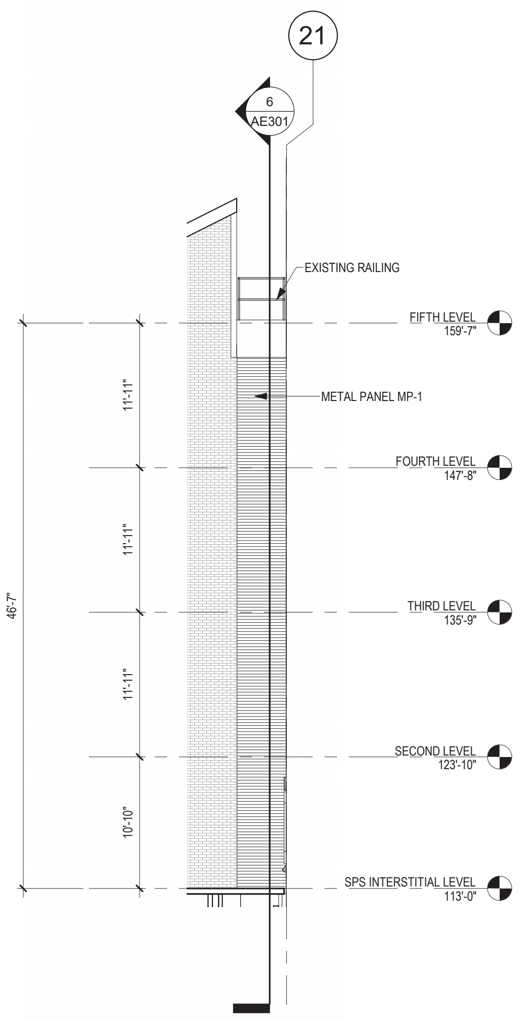
5 EXTERIOR ELEVATION - STAIR TOWER - EAST 1/8" = 1'-0"
