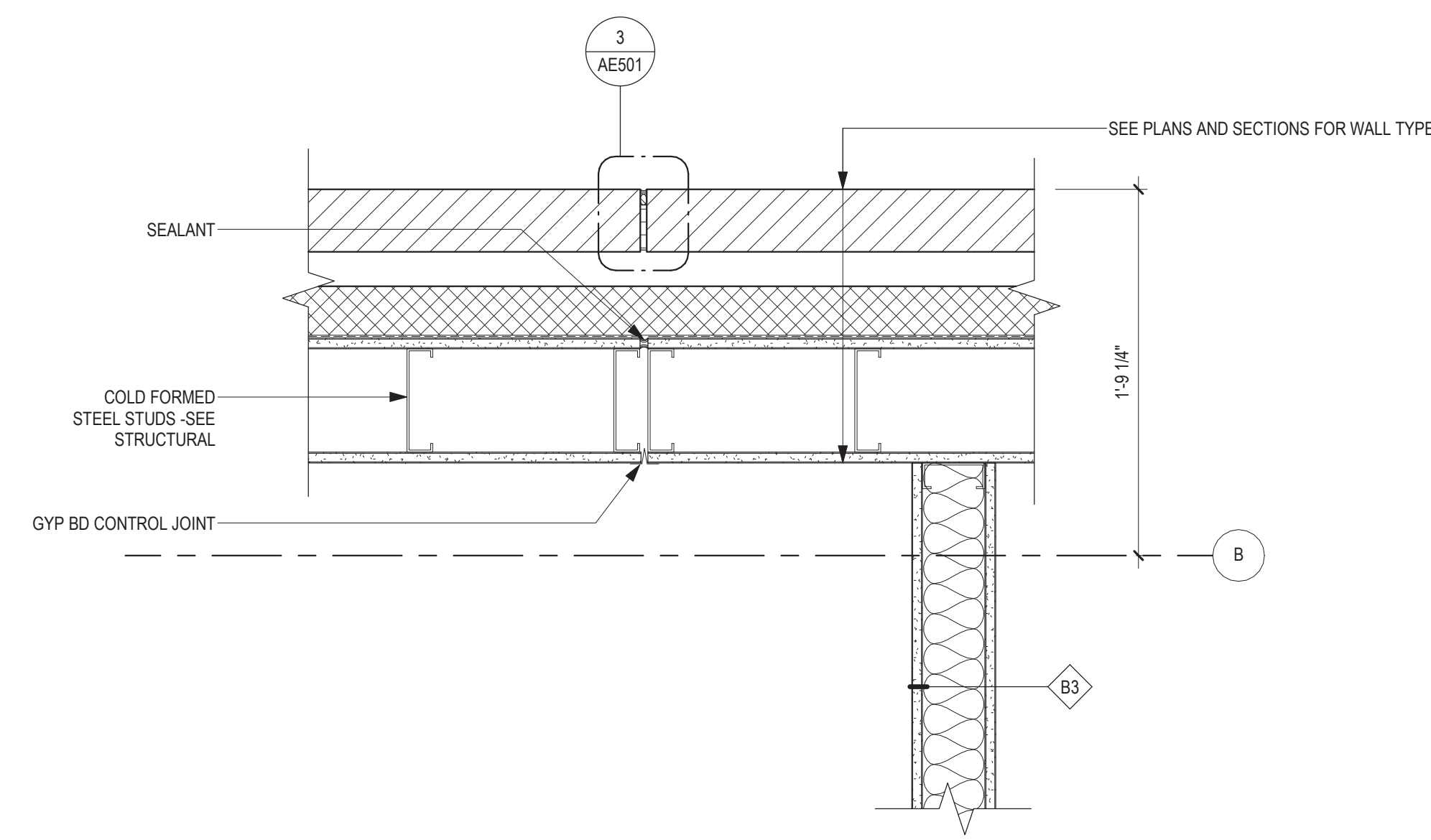
4 PLAN DETAIL - BRICK AND STEEL STUD ABOVE CAST IN PLACE CONCRETE TRANSITION 1 1/2" = 1'-0"
