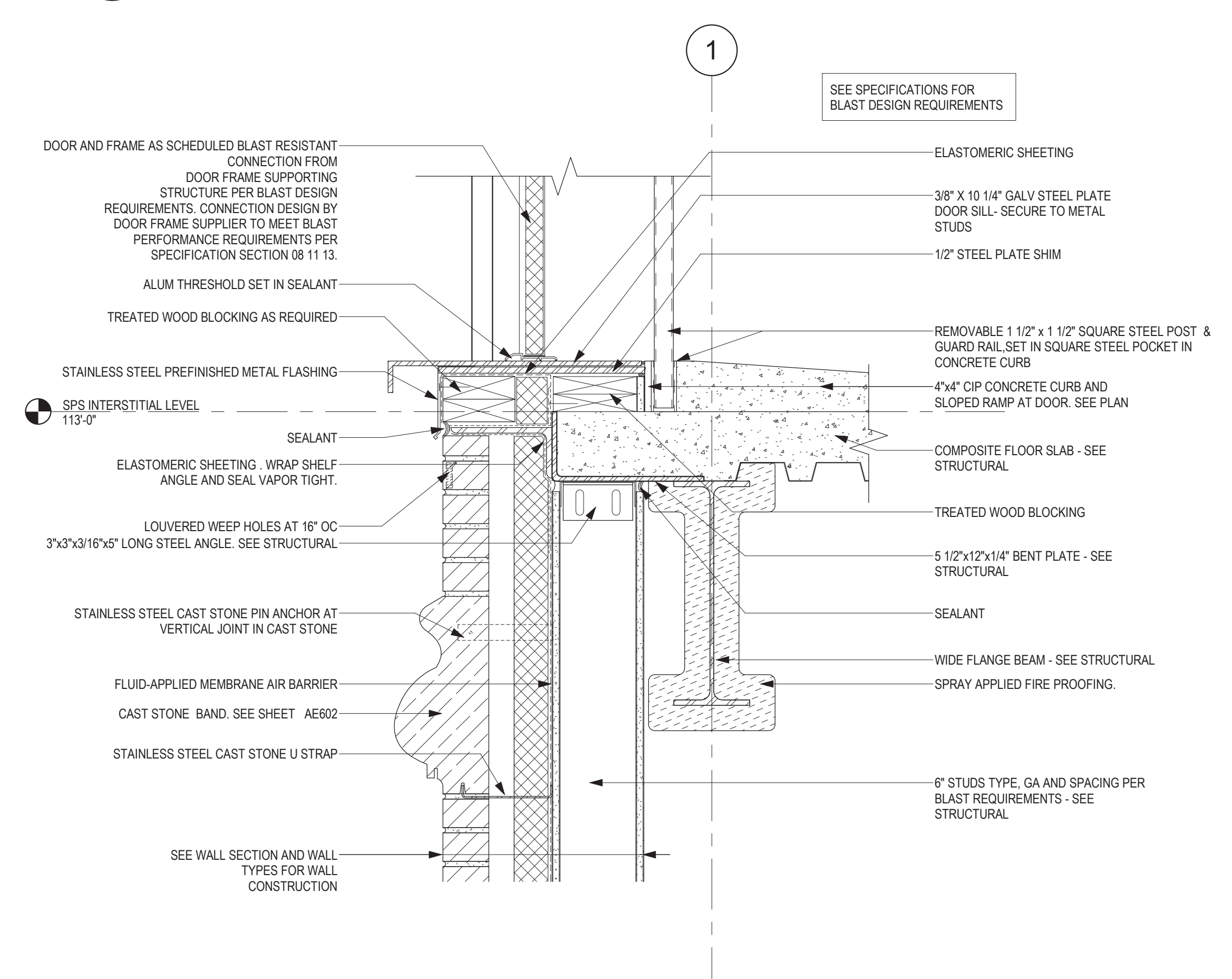
4 SECTION DETAIL - INTERSTITIAL DOOR SILL AND STONE BAND 1 1/2" = 1'-0"
