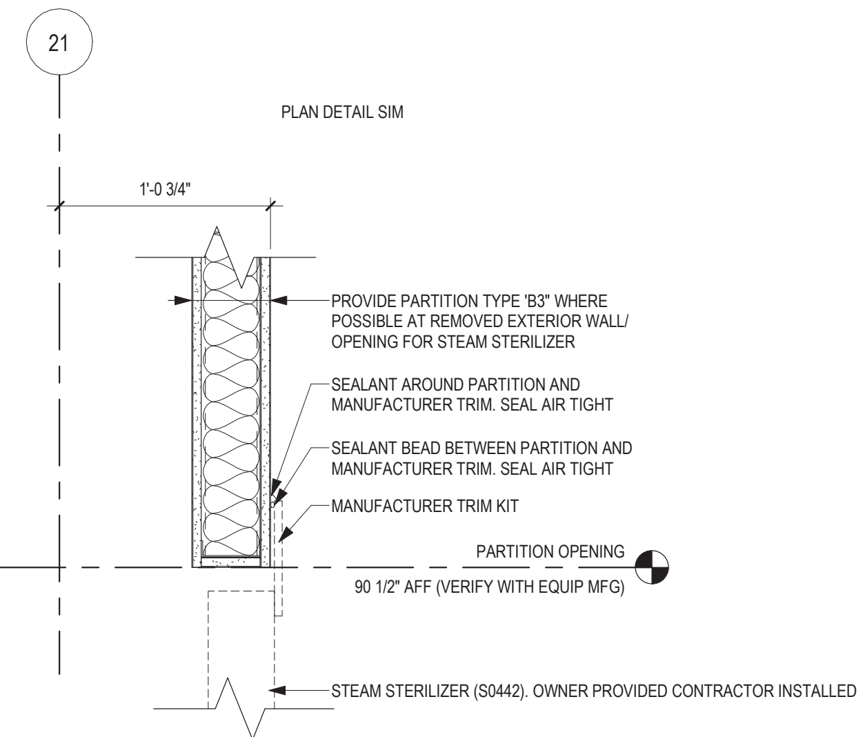
13 SECTION DETAIL - OPENING AT STEAM STERILIZER (TYP) 1 1/2" = 1'-0"
