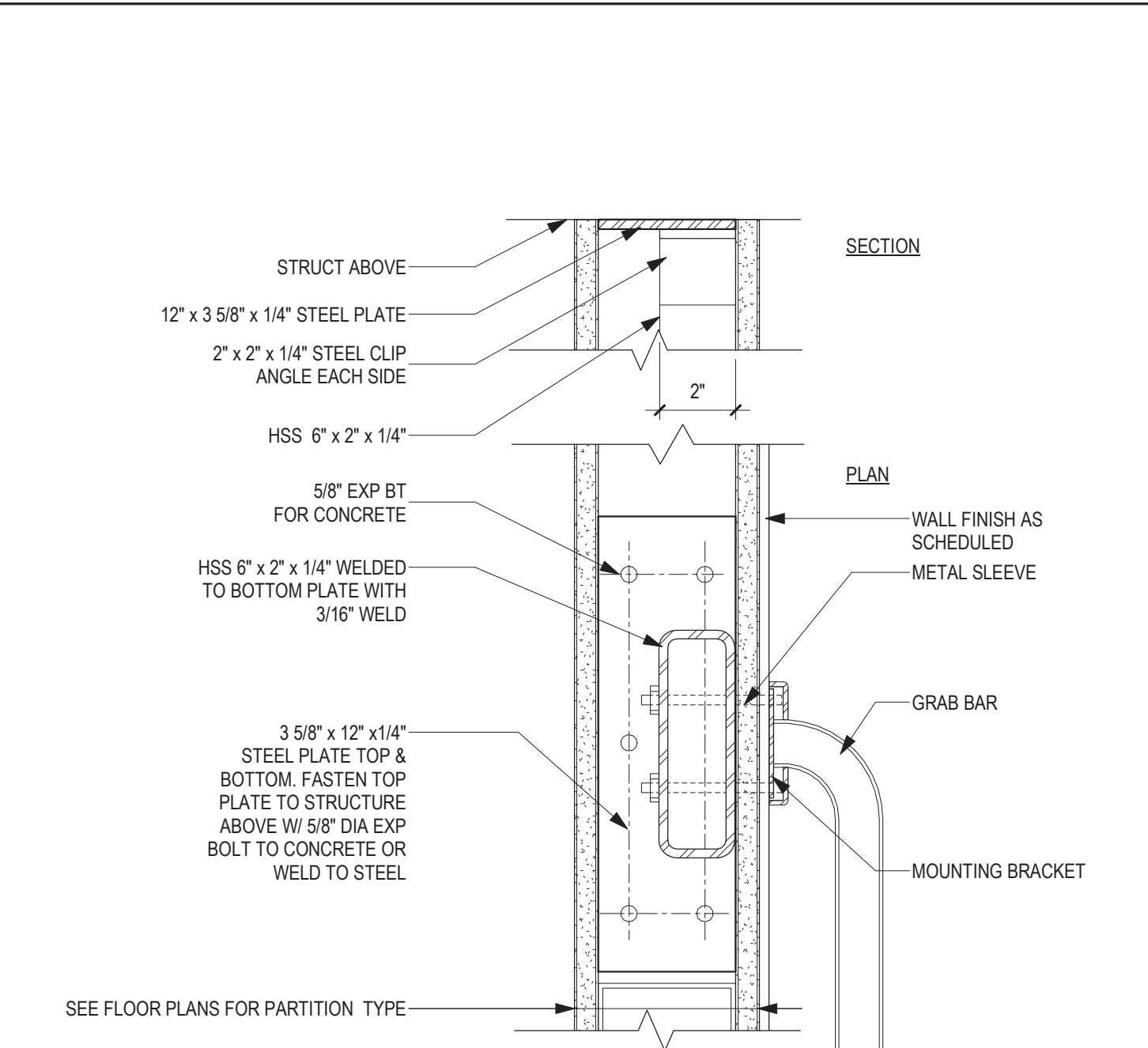
2 DETAIL - GRAB BAR SUPPORT - STEEL 3" = 1'-0"
