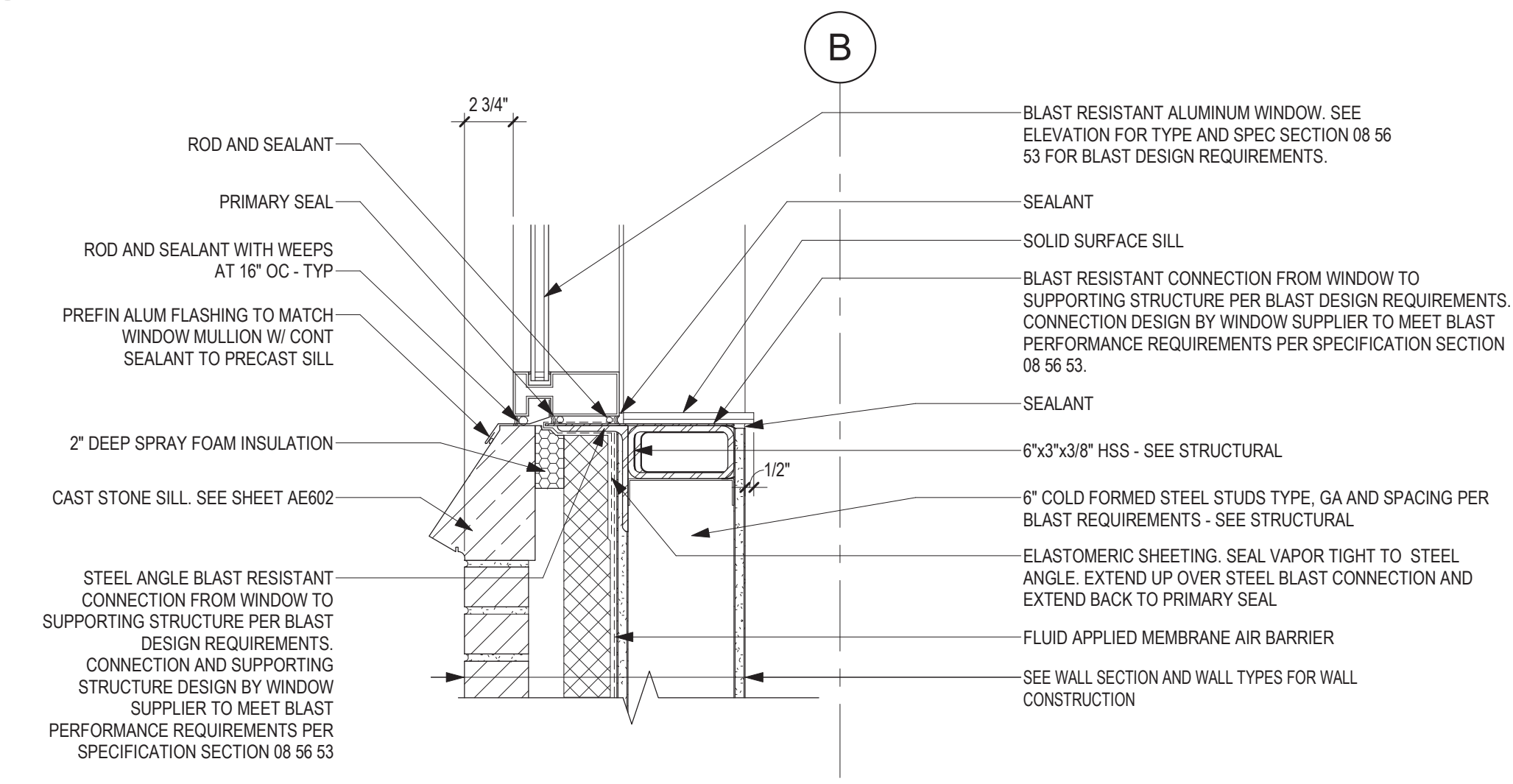
5 SECTION DETAIL - WINDOW SILL @ BRICK (TYP) 1 1/2" = 1'-0"
