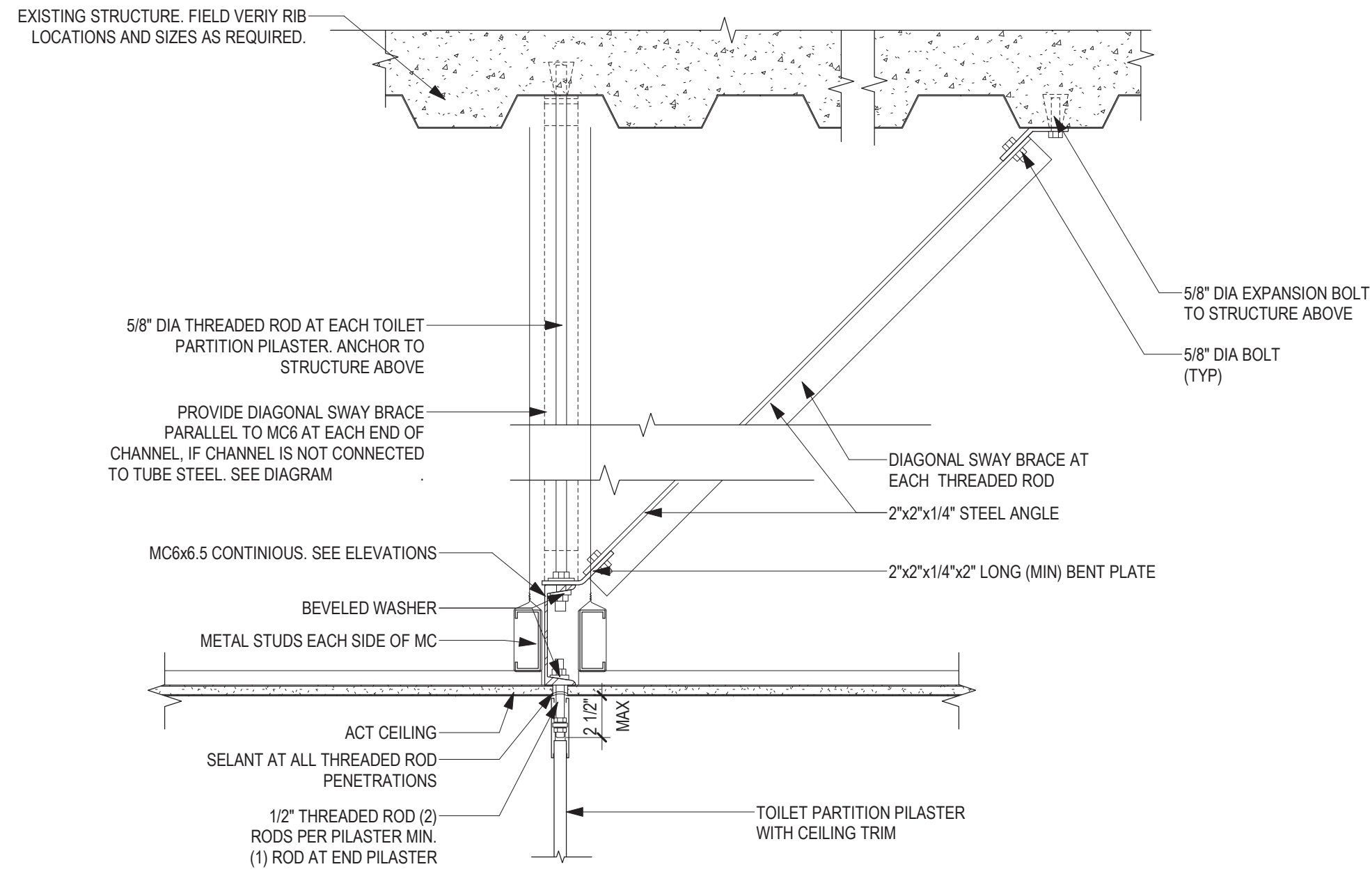
SECTION DETAIL - CEILING MOUNTED TOILET PARTITIONS 1 1/2" = 1'-0"
