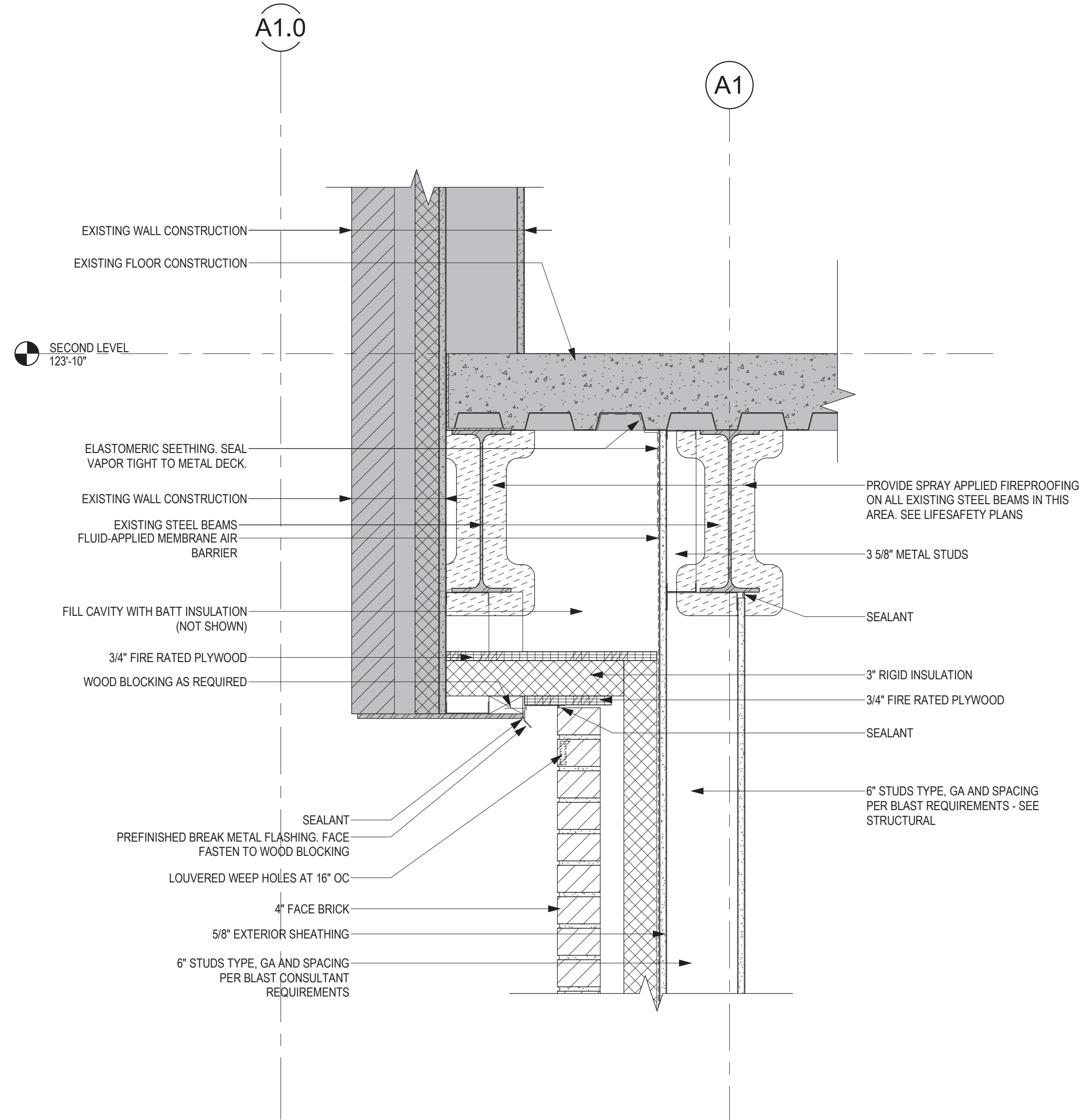
3 SECTION DETAIL - SOFFIT AT EXISTING ADDITION 1 1/2" = 1'-0"
