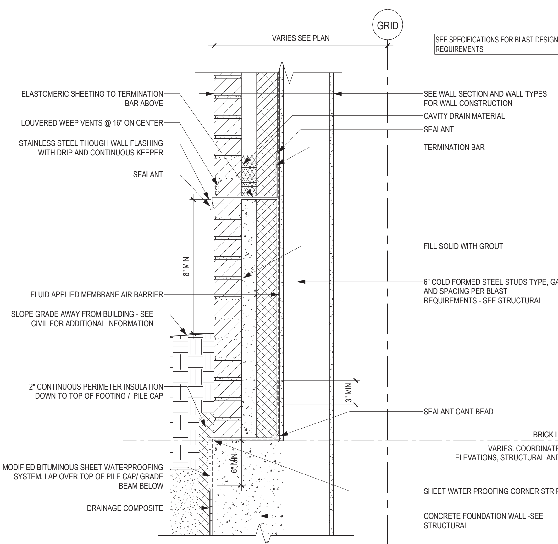
2 SECTION DETAIL - FACEBRICK AND METAL STUD AT GRADE 1 1/2" = 1'-0"
