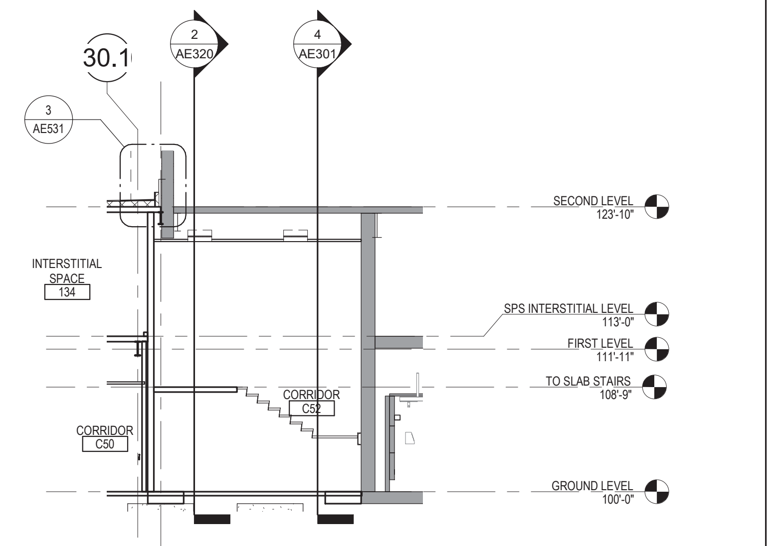
5 BUILDING SECTION - EXIT CORRIDOR @ EXISTING - NORTH / SOUTH 1/8" = 1'-0"
