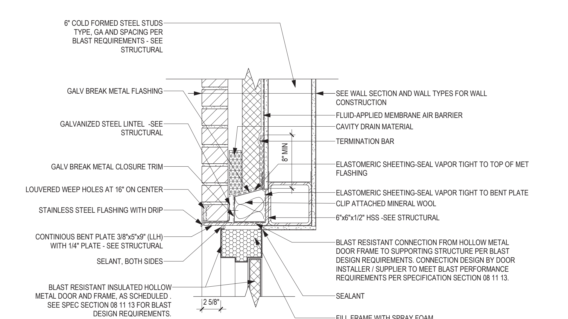
4 SECTION DETAIL - HM FRAME HEAD AT METAL STUD BACK UP AND FACE BRICK 1 1/2" = 1'-0"
