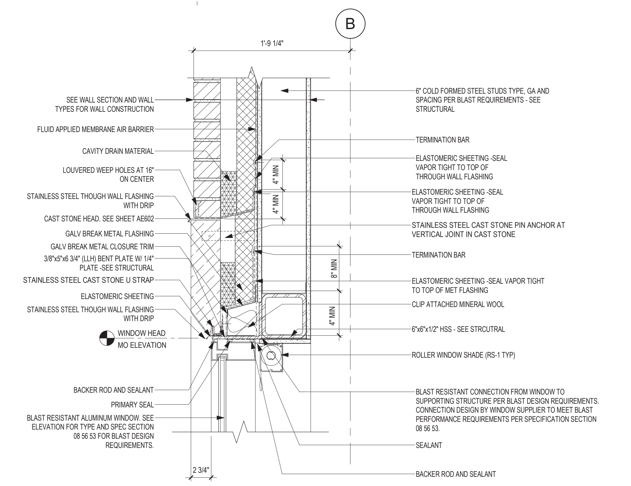
3 SECTION DETAIL - WINDOW HEAD @ BRICK (TYP) 1 1/2" = 1'-0"
