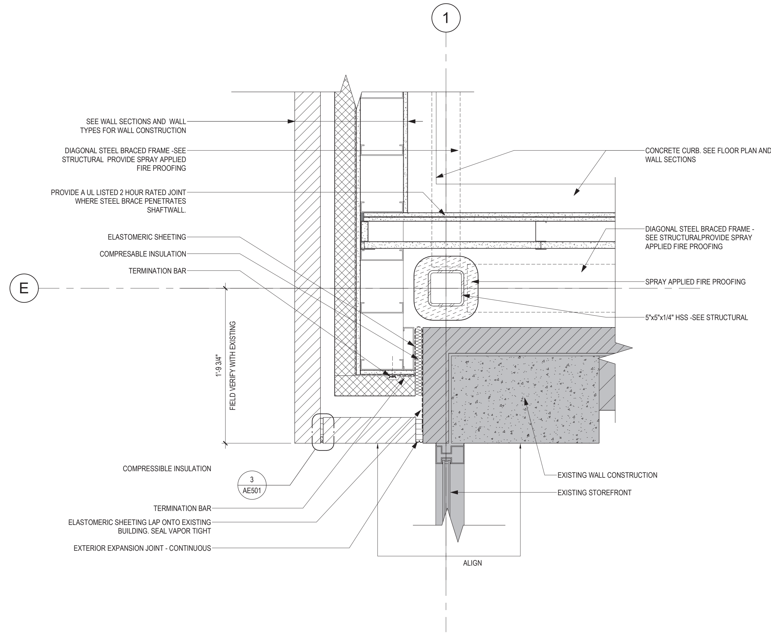
5 PLAN DETAIL - BRICK AND STEEL STUD AT EXISTING STAIR TOWER - INTERSTITIAL 134 1 1/2" = 1'-0"
