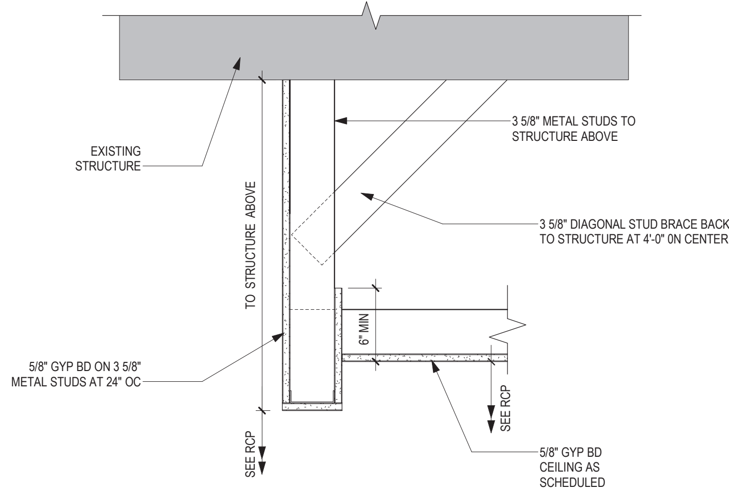
SECTION DETAIL - GYP BD RETURN 1 1/2" = 1'-0"
