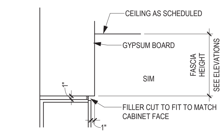
7 CASEWORK / LOCKERS AT GYP BD SOFFIT 3/4" = 1'-0"
