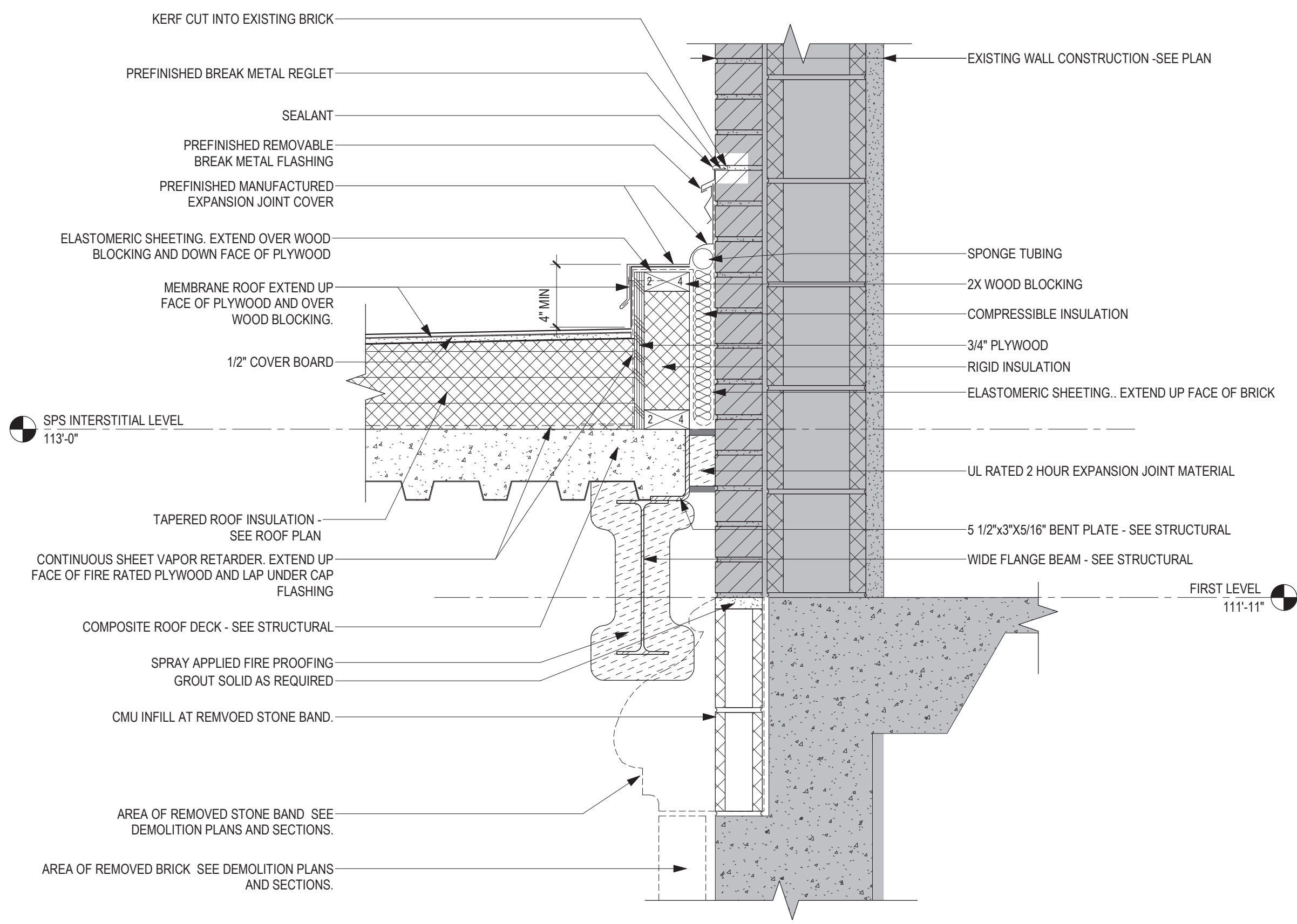
3 ROOF DETAIL - MEMBRANE ROOF @ EXISTING BRICK 1 1/2" = 1'-0"
