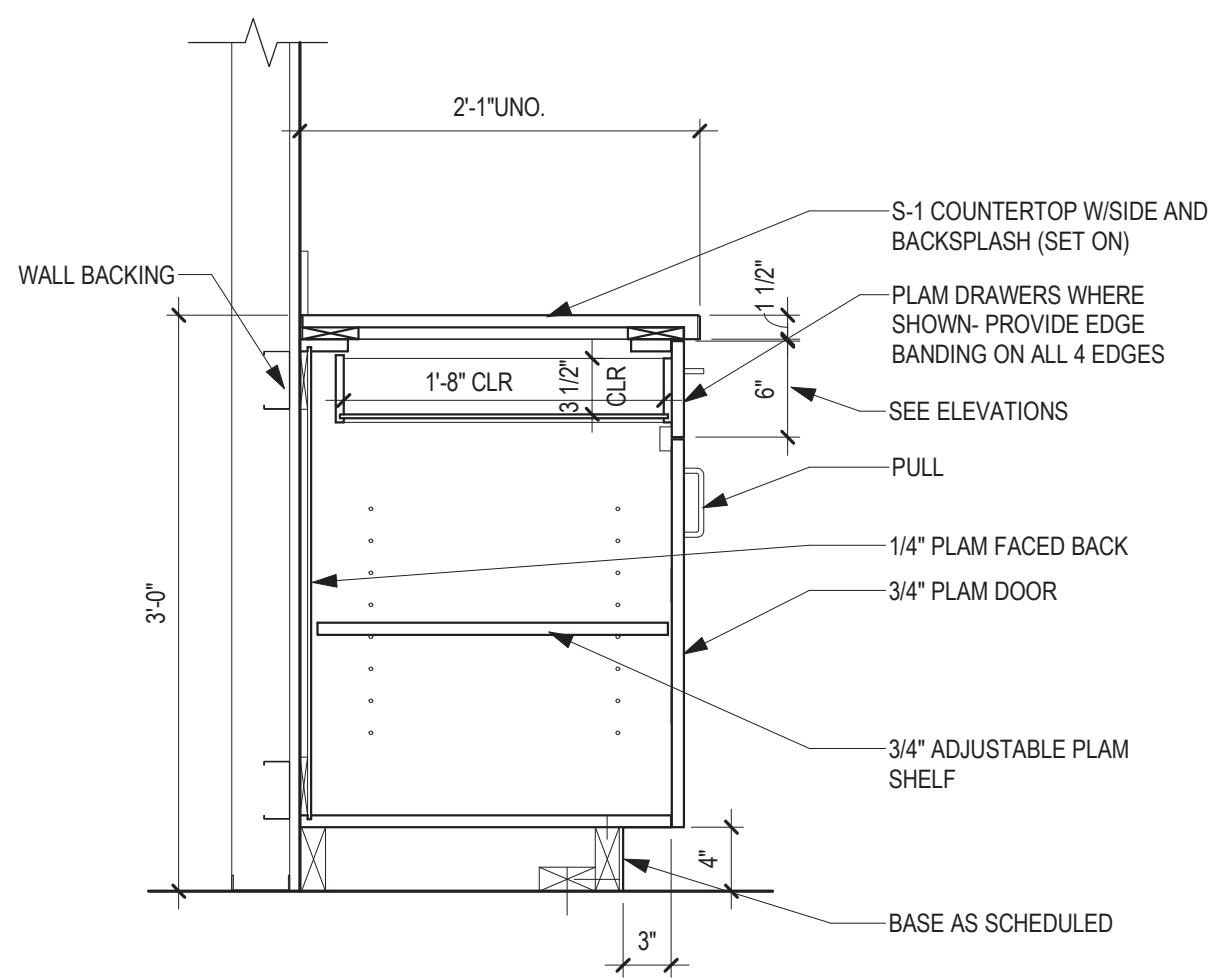
2 SECTION - BASE CABINET DRAWER & DOOR 1" = 1'-0"
