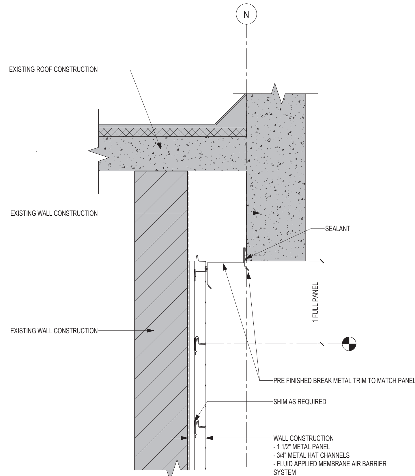
5 SECTION DETAIL - METAL PANEL AT PARAPET 1 1/2" = 1'-0"
