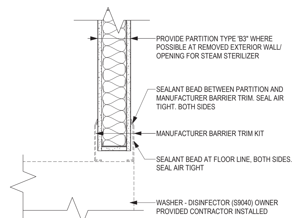
1 PLAN DETAIL - SST BARRIER FLANGE @ WASHER - DISINFECTOR 1 1/2" = 1'-0"
